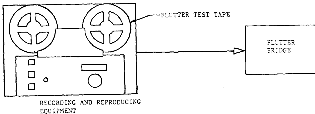
Figure 4 - Equipment Arrangement for Flutter and Wow Measurement
