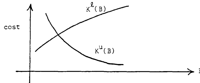
FIGURE 5. Minimum upper and lower echelon cost functions vs. B .
