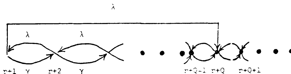
FIGURE 2. State transition flow diagram for inventory position
