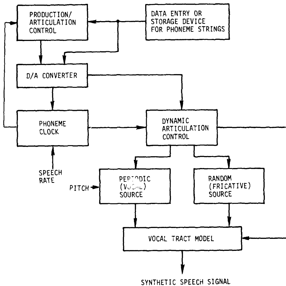
Figure 9. Block diagram of a VOTRAX phoneme synthesizer.
