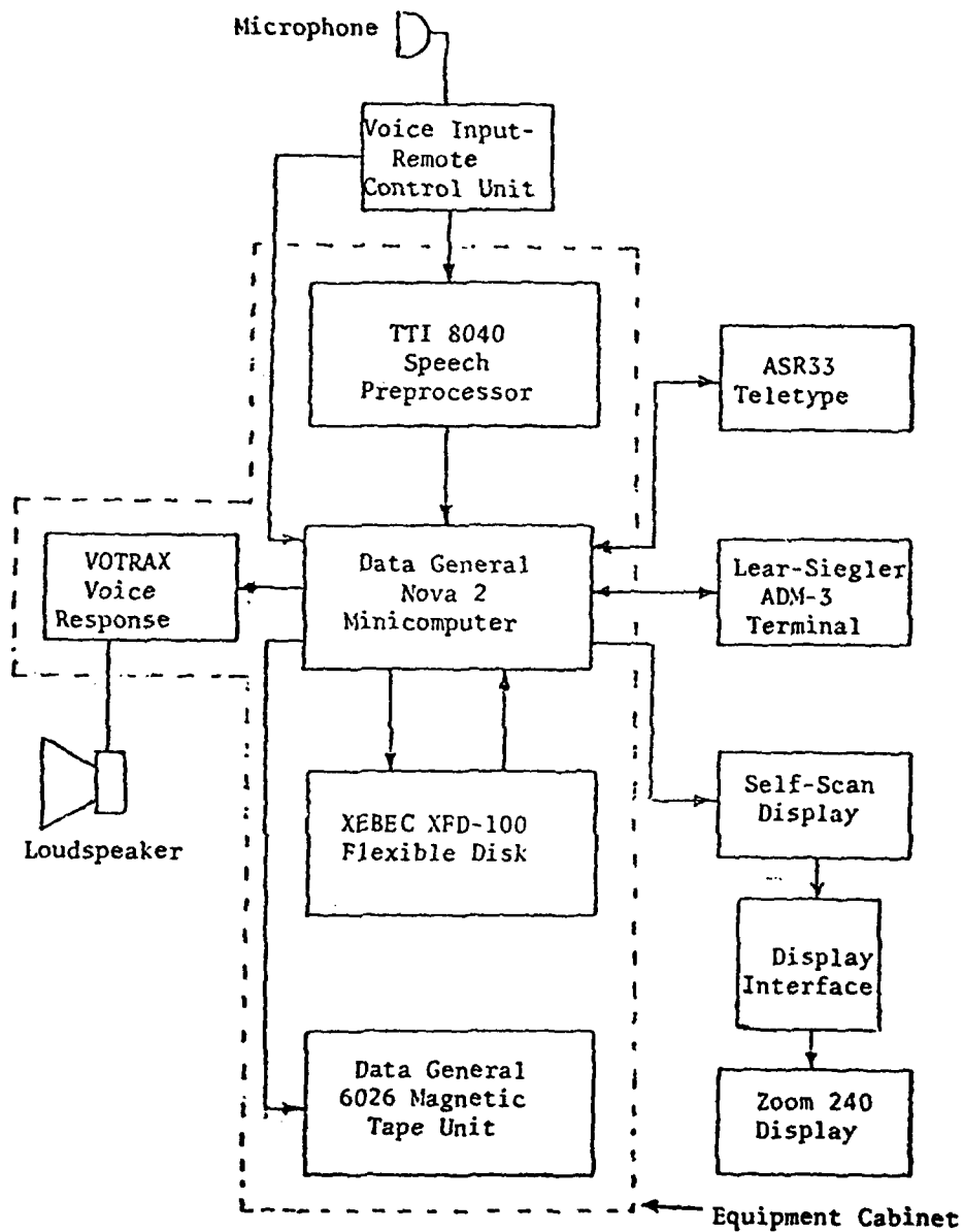
Figure 1. Block diagram of DLMS voice recognition system.
