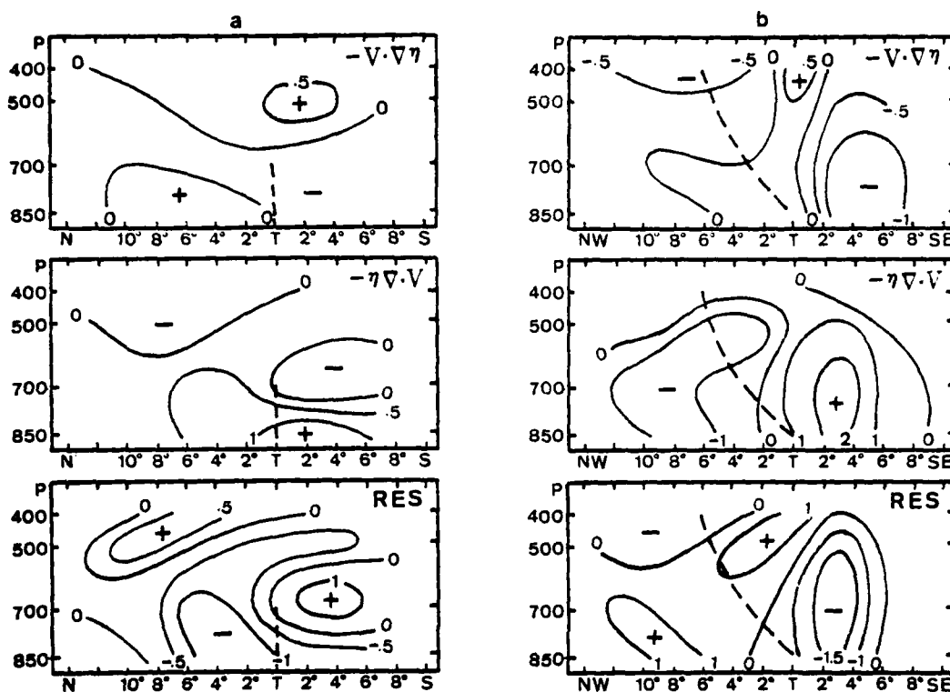
FIG. 9. As in Fig. 8 except for stage II.
