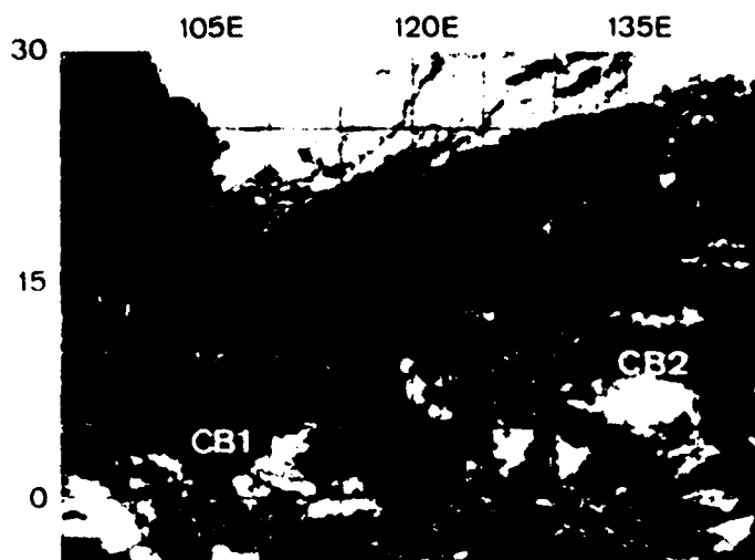
FIG. 3. NOAA-3 mosaic for 3 December 1974, centered near 0800 GMT.
