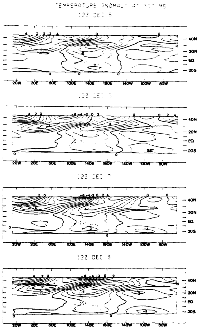
FIG. 4. As in Fig. 2 except for the temperature at 300 mb.
