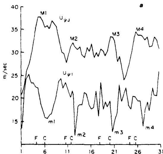
FIG. 12a. As in Fig. 11 except for the zonal component of the rotational part of the wind ( -\partial\psi/\partial y ) averaged over the area U_{\psi J} and U_{\psi I} indicated in Fig. 5.
