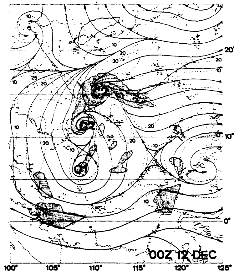
FIG. 13. As in Fig. 2 except for 0000 GMT 12 December 1974.
