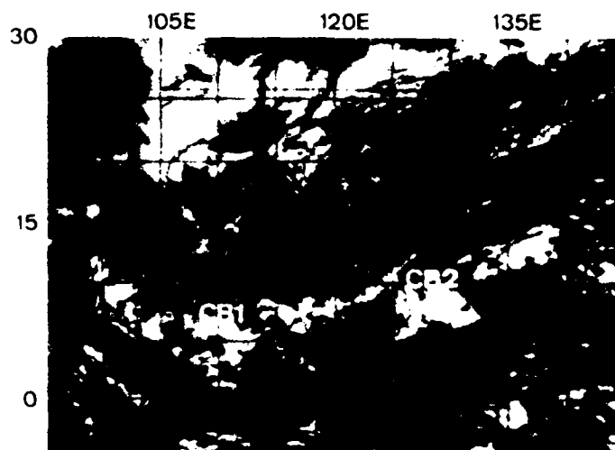
FIG. 4. NOAA-3 mosaic for 6 December 1974, centered near 0800 GMT.
