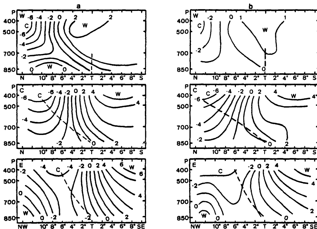
FIG. 5. As in Fig. 4 except for T' ( ^{\circ}\text{C} ).
