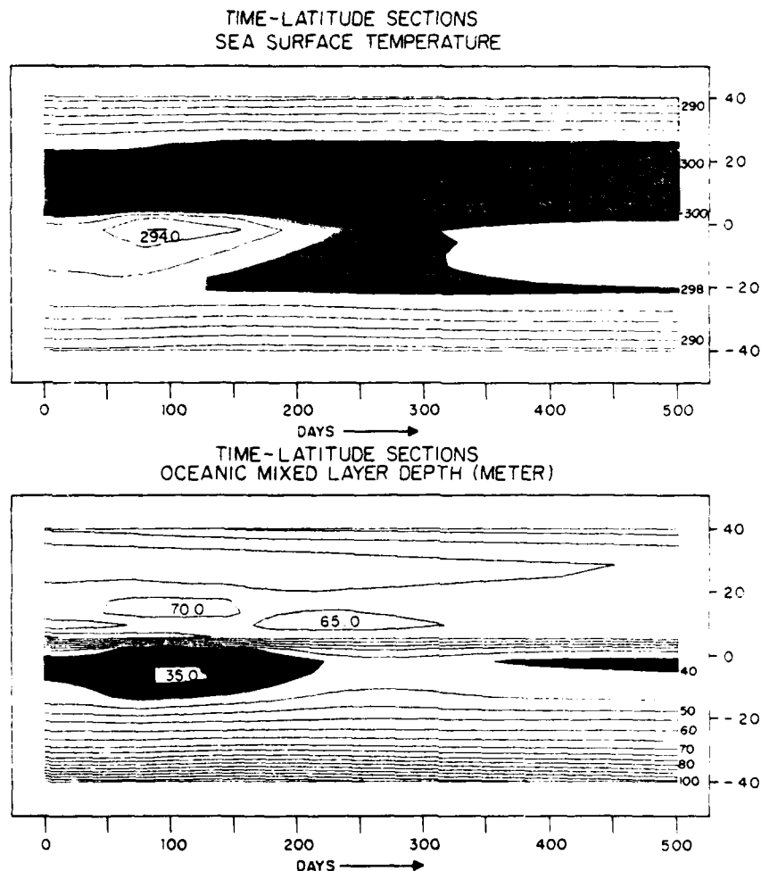
FIG. 16. Time-latitude section of the ocean mixed layer temperature and depth as a result of the perturbation, for the same period as in Fig. 12.
