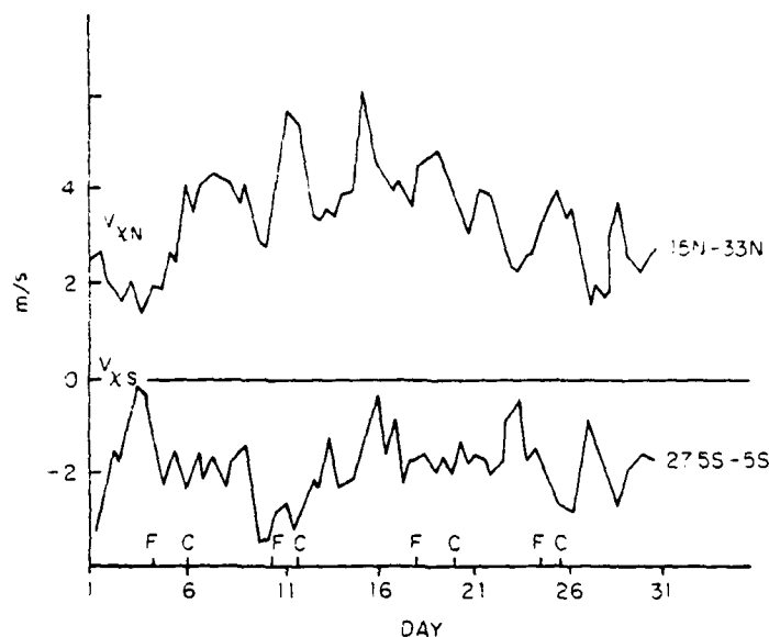
FIG. 8. Time-series of the meridional component of the divergent part of the wind ( -\partial v / \partial y ) averaged over the area indicated by V_{XN} and V_{XS} in Fig. 5.
