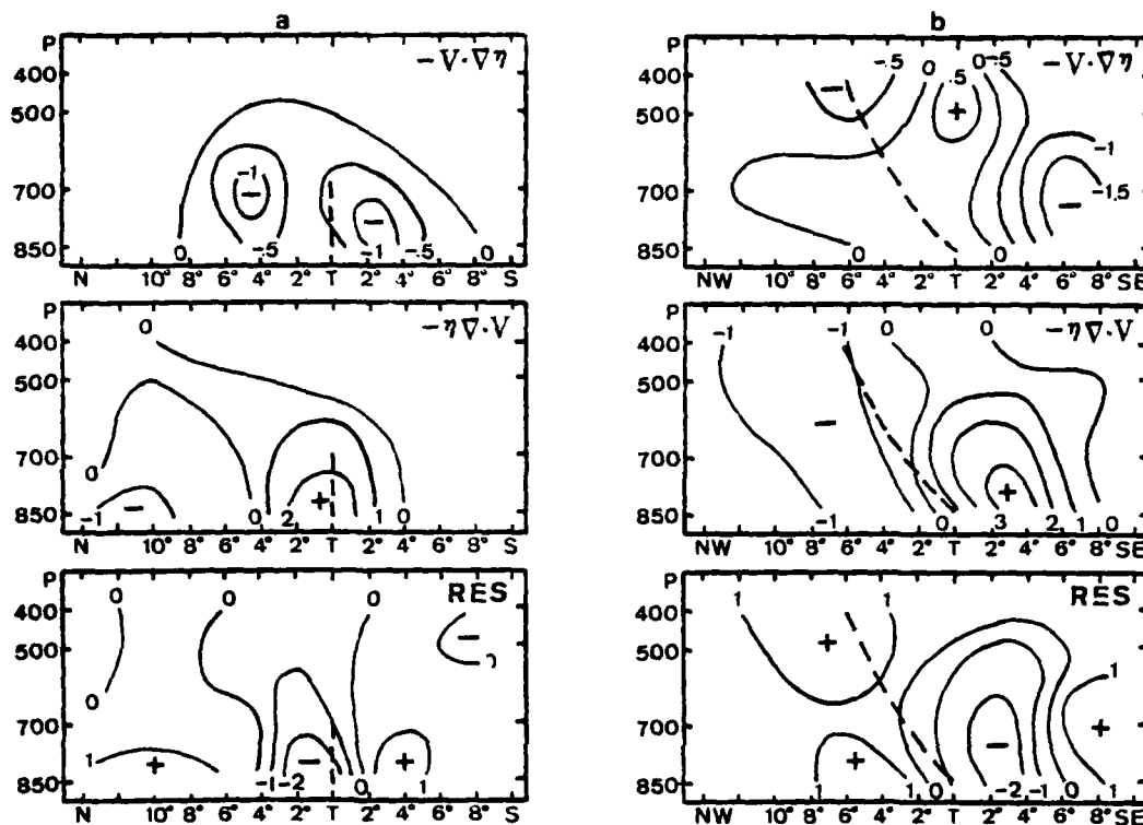
FIG. 8. Vertical cross sections of horizontal vorticity advection, divergence and residual terms during stage I in (a) section W and (b) section E. Units are 10^{-7} \text{ s}^{-1} (12 \text{ h})^{-1} . Dashed lines indicate the trough axes. The abscissa is distance in degree latitude.
