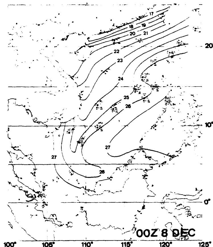
FIG. 8. Surface temperature analysis for 0000 GMT 8 December 1974.
