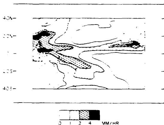
FIG. 1. Satellite-derived annually averaged precipitation rates compiled from Rao et al. (1976).
