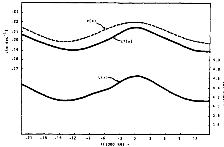
FIG. 21. As in Fig. 20 except for y=0 .
