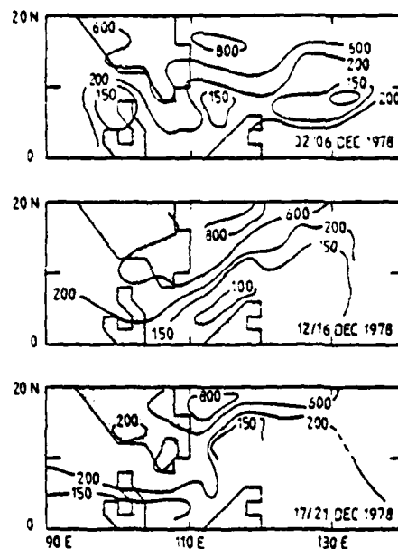
FIG. 2. Isopleths of cloud-top heights for the periods 2–6, 12–16 and 17–21 December 1978 (units: mb).
