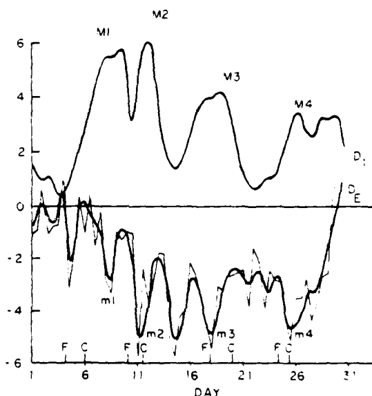
FIG. 9. As in Fig. 8 except for the area-averaged divergence over D_1 . The curve for D_E is included for comparison.
