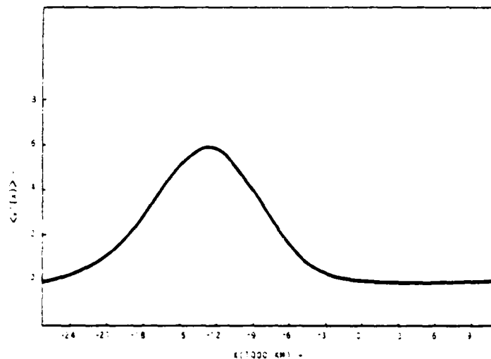
FIG. 7. Experiment 1: wave packet envelope \psi'(x) from the complete numerical model.
