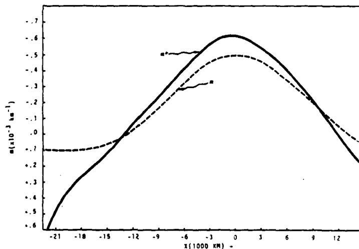
FIG. 13. Experiment 1: spatial growth rates n(x) from the parallel flow model and n^*(x) from the complete numerical model. When n < 0 there is downstream growth.
