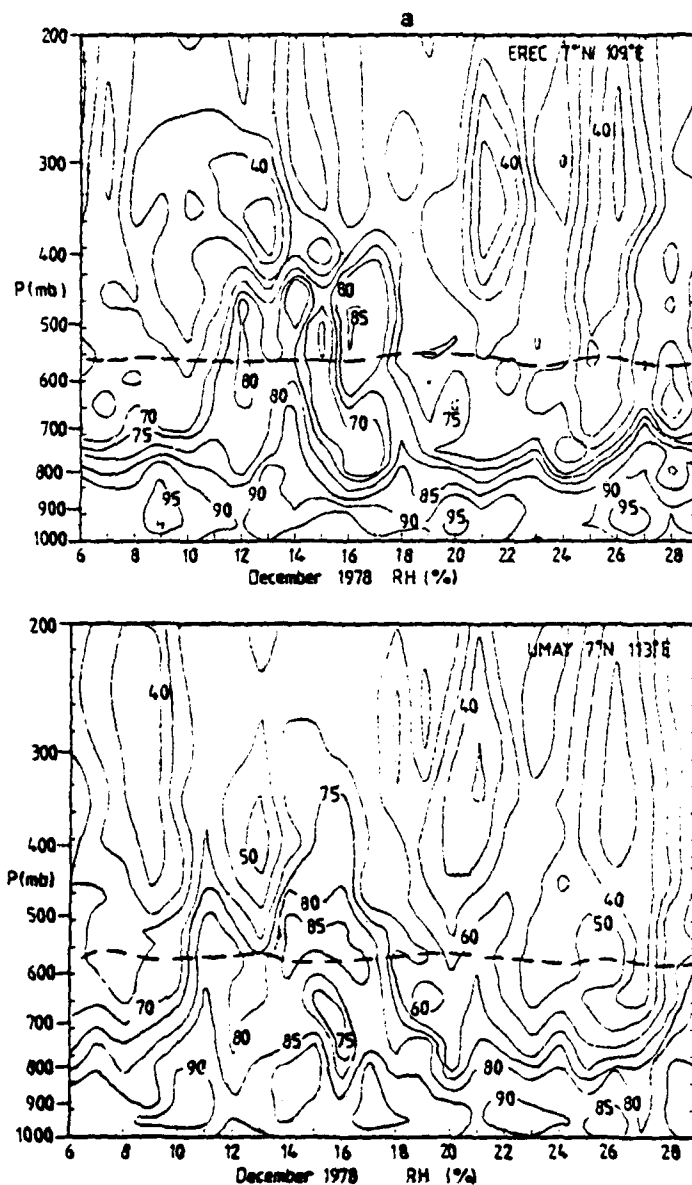
FIG. 3. (a) Time sections of relative humidity against pressure height for the three USSR ships located in the South China Sea during Phase I of WMONEX between 6–31 December 1978. The 0°C isopleth is shown as a dashed line. (b) As in Fig. 3a except for equivalent potential temperature (units: K).
