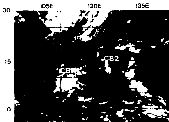
FIG. 9. NOAA-3 mosaic for 9 December 1974, centered near 0800 GMT.
