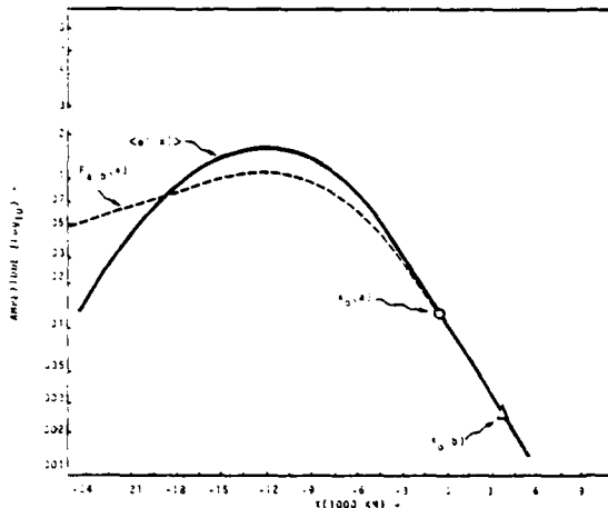
FIG. 17. Experiment 2: the wave packet envelopes. F_0(x) is from the analytical model for initial point x_0(a) = -375 km, F_0(x) is from the analytical model for initial point x_0(b) = 3750 km, and \langle\psi'(x)\rangle is from the complete numerical model.
