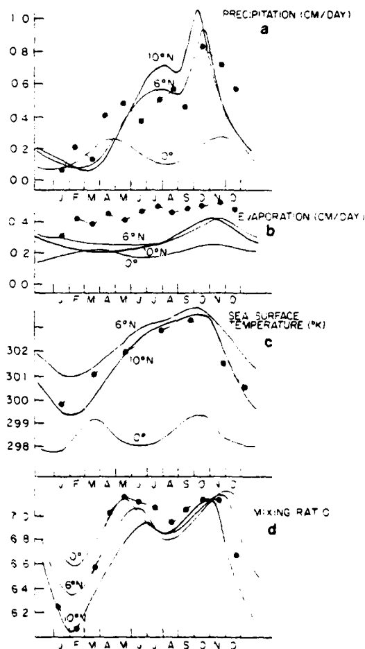
FIG. 9. CPAC time series of (a) precipitation rate, (b) evaporation, (c) SST and (d) mixing ratio at 750 mb at different latitudes for the fourth year of the simulated seasonal cycle. Observed monthly averages denoted by black dots are for the tropical central Pacific and are compiled from (a) Rao et al. (1976), (b) Newell et al. (1972), (c) Alexander and Mobley (1976) and (d) Newell et al. (1972).
