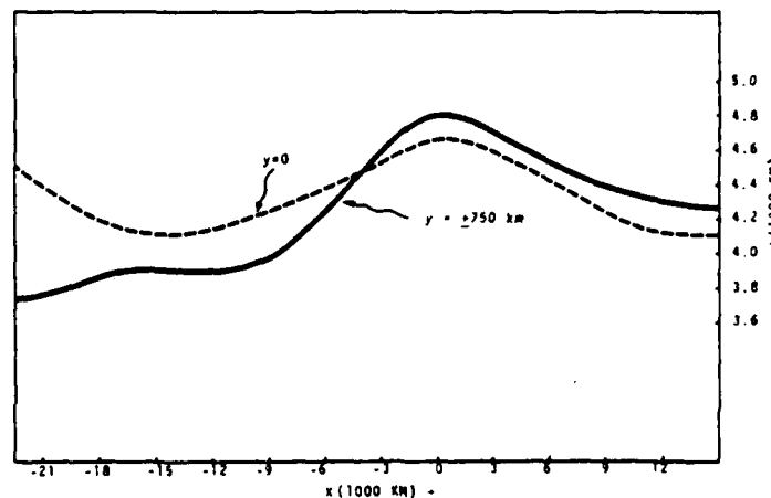
FIG. 22. Experiment 2: wavelengths L(x) from the complete numerical model for y=0 and y=-750 km.
