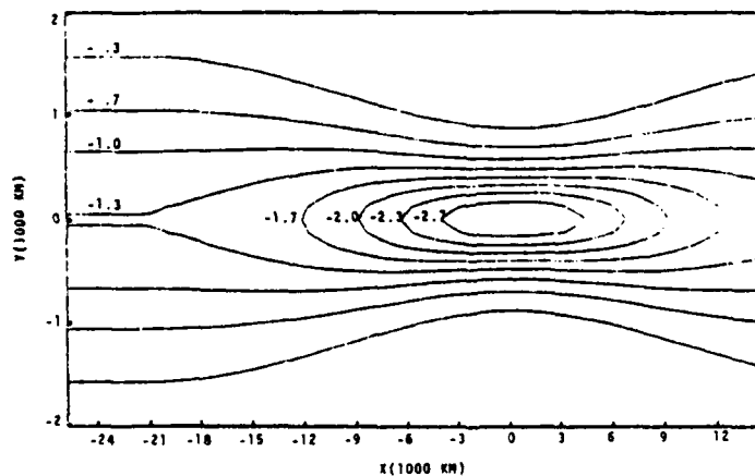
FIG. 2. Experiment 1: the u(x, y) field (units, 10 \text{ m s}^{-1} ).
