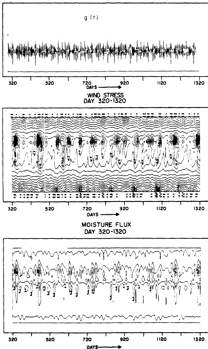
FIG. 18. Time-latitude section of the wind stress ( 10^{-1} \text{ N m}^{-2} ) and surface moisture flux ( \text{cm day}^{-1} ) from the ocean as a result of continuous short-period atmospheric forcings for the last 3 years of the integration period. Data taken from every 5 days in the time series.
