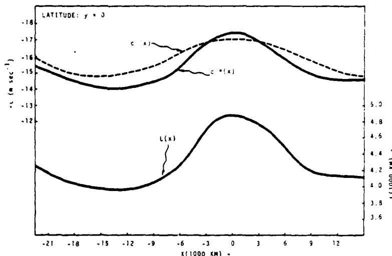
FIG. 12. As in Fig. 11 except for y=0 .
