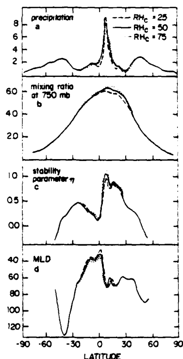
FIG. 11. Latitudinal distribution of (a) precipitation ( \text{cm day}^{-1} ), (b) mixing ratio at 750 mb ( 10^{-1} \text{ g kg}^{-1} ), (c) stability parameter \eta and (d) MLD (m) for different values of critical relative humidity RH_c .
