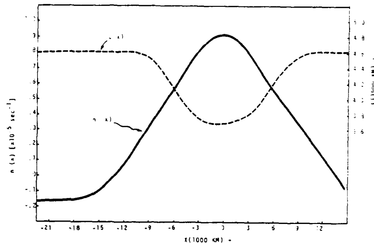
FIG. 3. The most unstable wavelength L(x) and the corresponding local growth rate n(x) determined from the parallel flow model.
