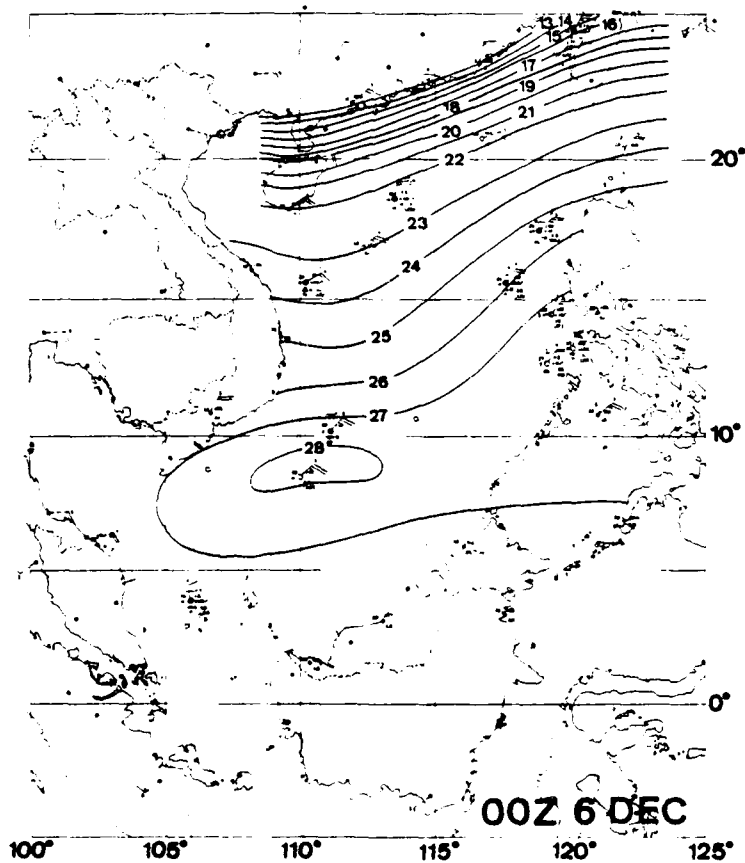
FIG. 5. Surface temperature analysis for 0000 GMT 6 December 1974.
