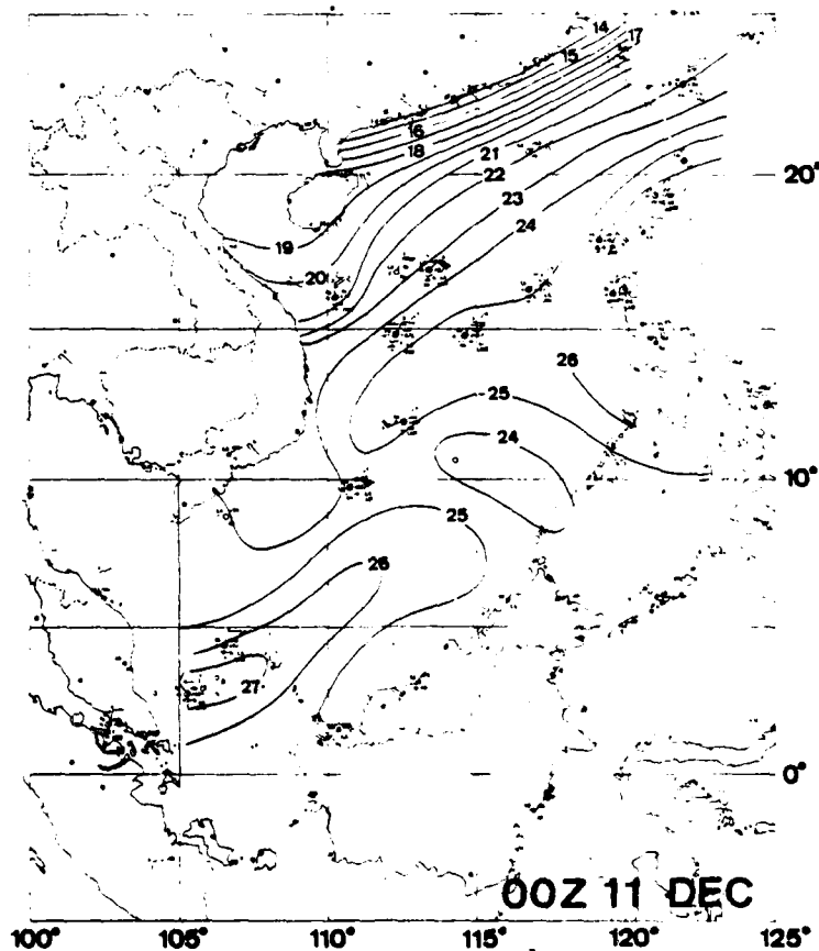
FIG. 12. Surface temperature analysis for 0000 GMT 11 December 1974.
