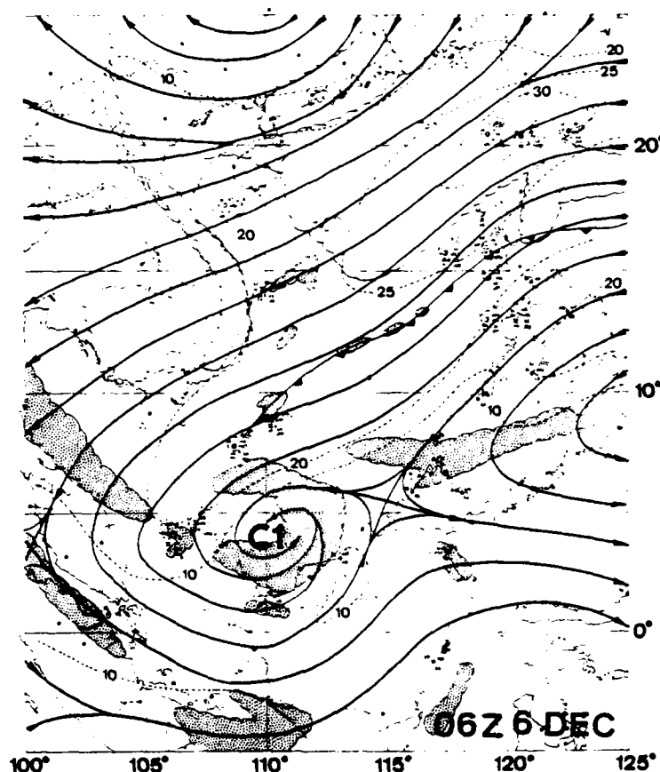
FIG. 6. As in Fig. 2 except for 0600 GMT 6 December 1974.
