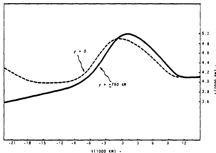
FIG. 8. Experiment 1: wavelengths L(x) from the complete numerical model for y = 0 and y = -750 km.
