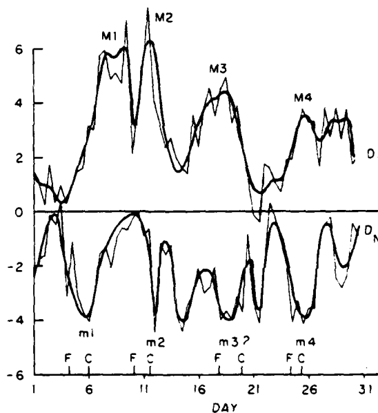
FIG. 6. Area-averaged divergence over regions D_1 and D_4 in units of 10^{-4} \text{ s}^{-1} . Twice daily values are indicated by thin lines and the best fitting curves by heavy lines. The symbols M1-4 and m1-4 denote respectively the maxima and minima in D_1 and D_4 corresponding to the major cold surges of the month. On the horizontal axis, the letters F and C denote dates of frontal passage and recorded minimum surface temperature in Hong Kong.
