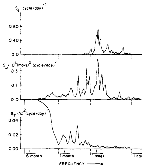
FIG. 20. Frequency spectra of the forcing function ( S_f ), the vertical p -velocity at 500 mb ( S_w ) and the SST ( S_T ) averaged over the southern tropics ( 0-10^\circ\text{S} ) from time series of a 1500-day simulated period.
