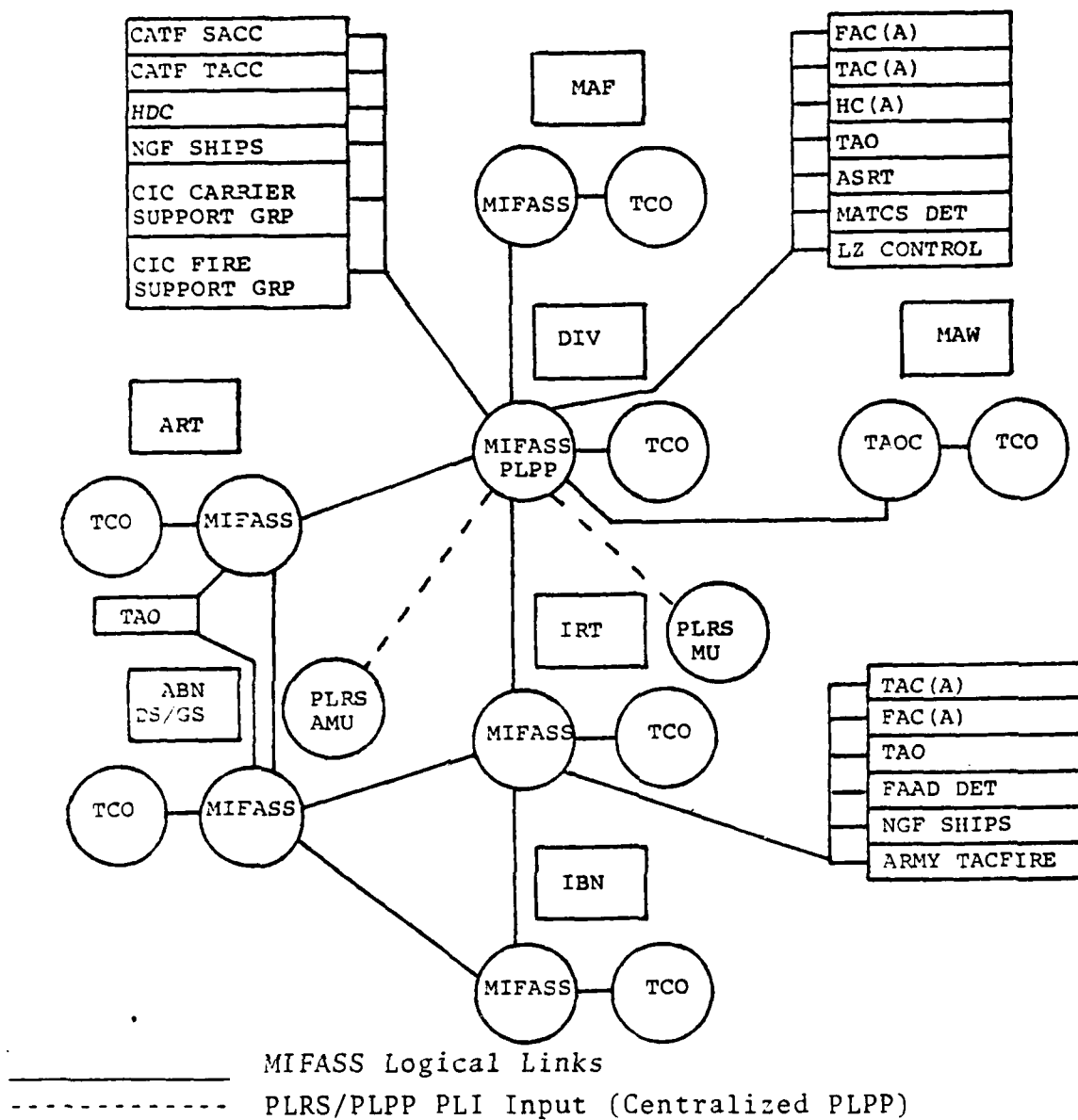
Figure (3) MIFASS Logical Interfaces And Information Flow
