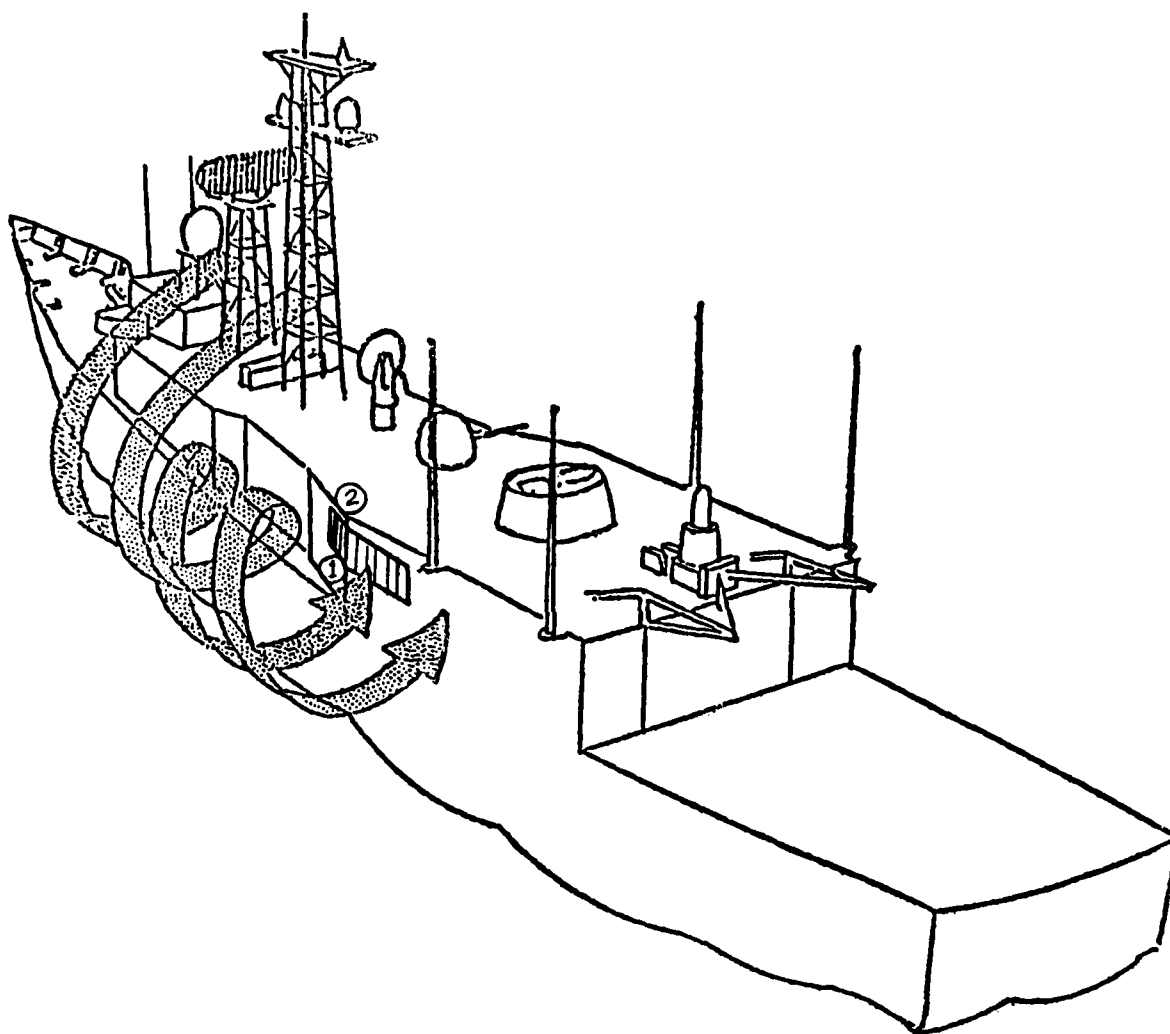
Fig. 2 — DTNSRDC wind tunnel model lee vortex. At-sea survey found 2.5X more salt loading on lee than upwind side. Instruments were mounted at 1 and 2 plus inside drop space and downstream of filters.
