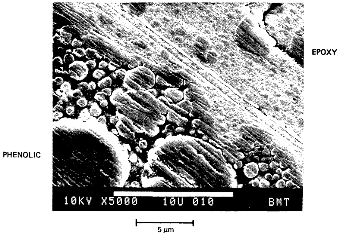
Figure 27. Boundary Between Nitrile-Phenolic and Epoxy Layers of FM-61
