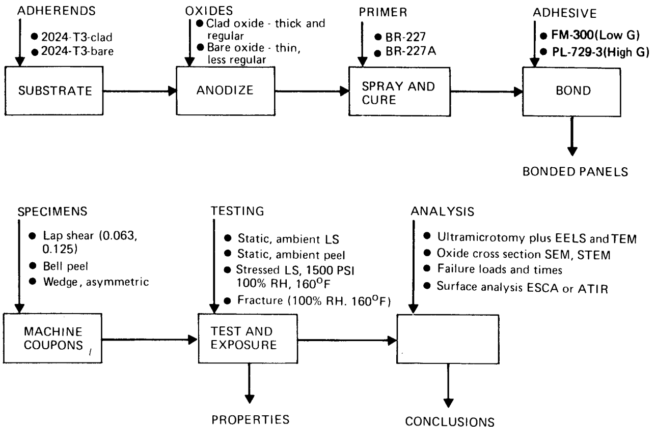
Figure 7. Task IV Test Plan
