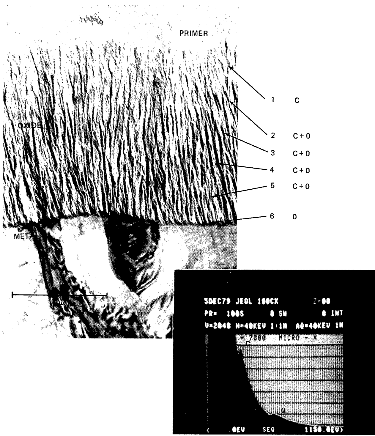
Figure 10. TEM Photomicrograph of a Thin Section of 2024-T3-Clad PAA with BR-227 Primer, Inset is an EELS Spectrum from Region 3
