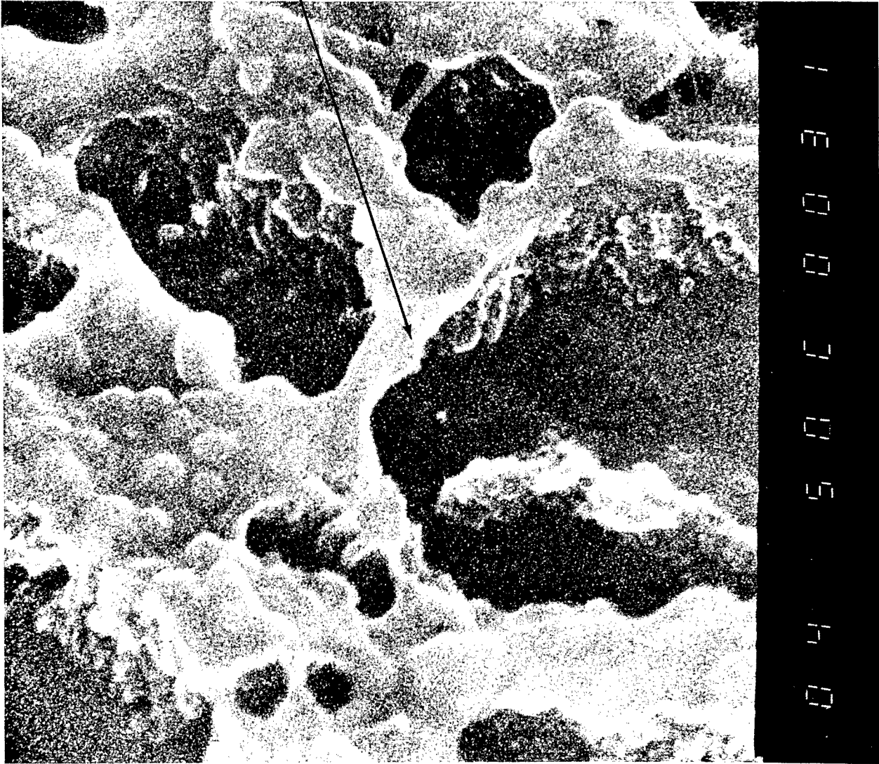
Figure 36. Transverse View of Failed Specimen—2024-T3-Bare, PAA Oxide, BR-227A Primer, FM-61 Adhesive
