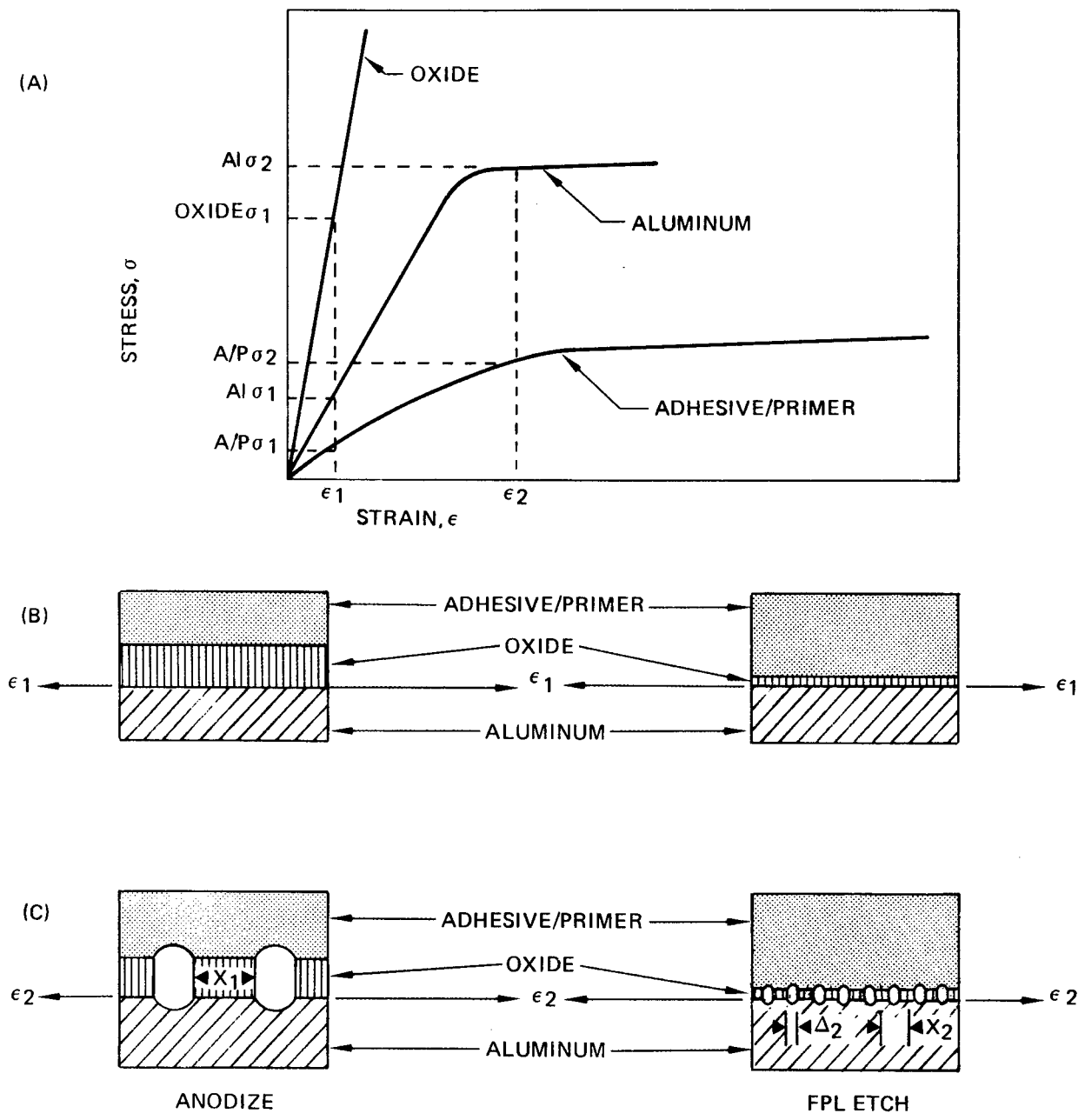
Illustration of how the stress-strain characteristics of the different components in a bonded system influence failure: (A) relative stress-strain characteristics of the three components; (B) system at strain, \epsilon ; and (C) system at strain \epsilon_2 where oxide has failed.
