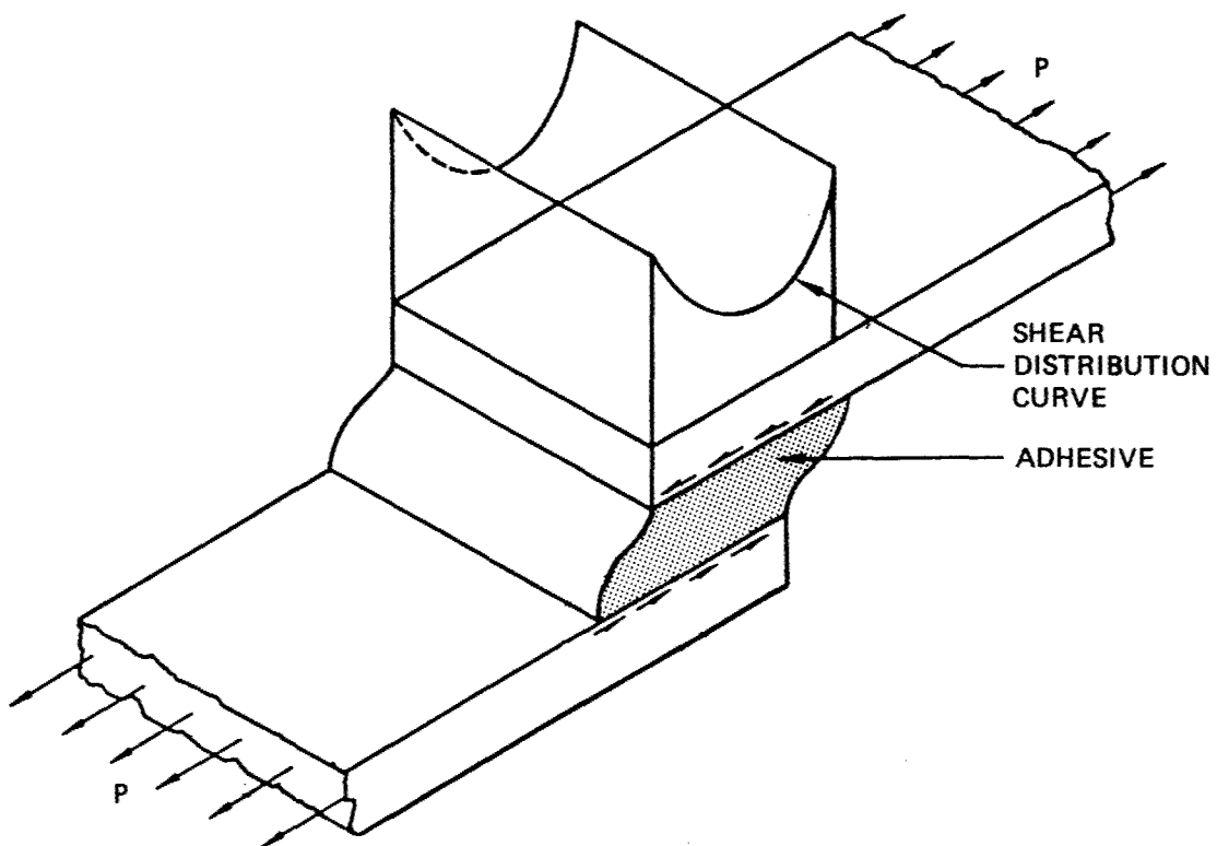
Figure 47. Lap Joint
