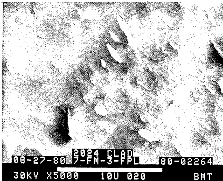
Figure 54. Failure Surface of BR-227/FM-300 on 2024-T3-Clad FPL
