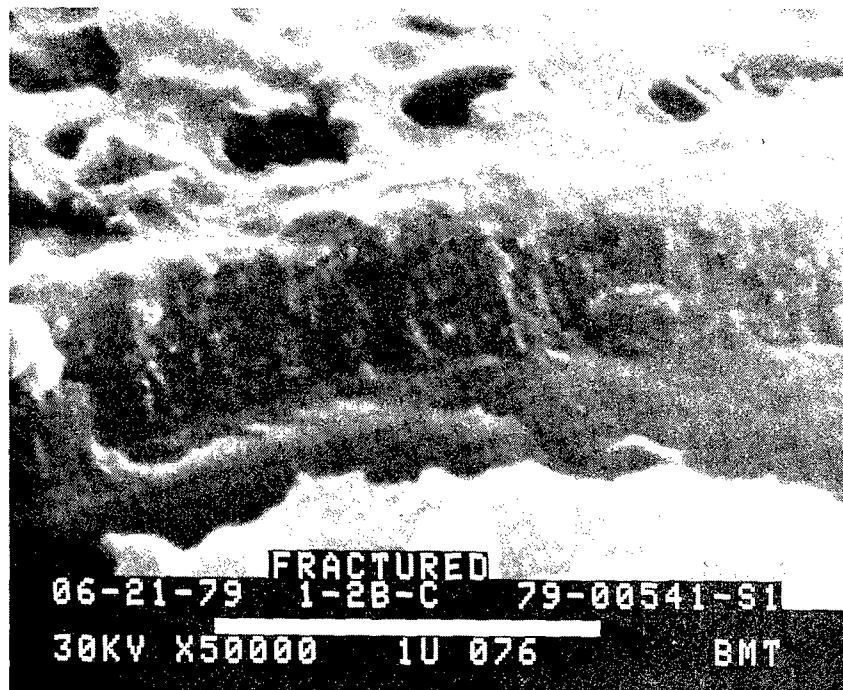
Figure 41. Transverse View of PL-728/PL-729-3 Failure Surface on 2024-T3-Bare PAA
