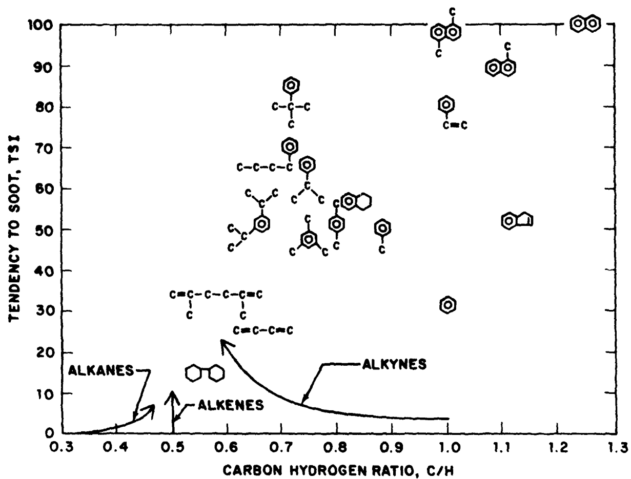
Figure 4. Effect of Molecular Structure on Tendency to Soot in Diffusion Flames
