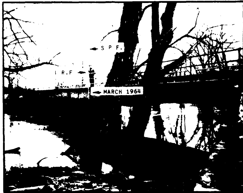
Figure 17 - Arrows indicate the heights of the Standard Project, Intermediate Regional, and March 1964 floods at the upstream side of Oxbow Road bridge, stream mile 7.04.
