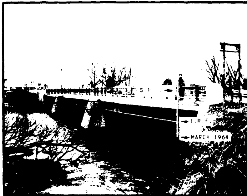
Figure 15 - Arrows indicate the heights of the Standard Project, Intermediate Regional, and March 1964 floods at the upstream side of N.Y.S. Route 31 bridge, stream mile 3.5.
