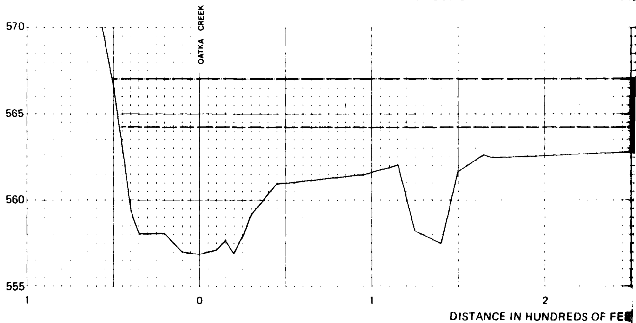
CROSS SECTION NO. 32 MILE PO
