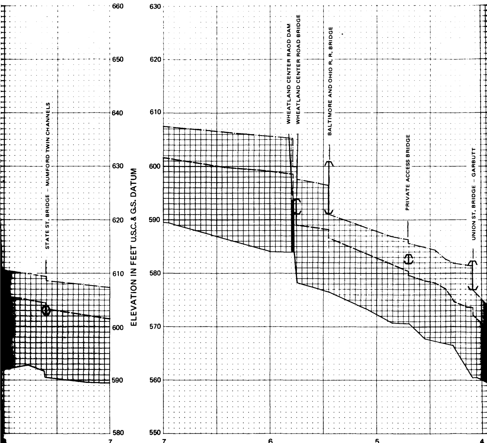
MILES UPSTREAM OF MOUTH OATKA CREEK FLOOD PROFILE
