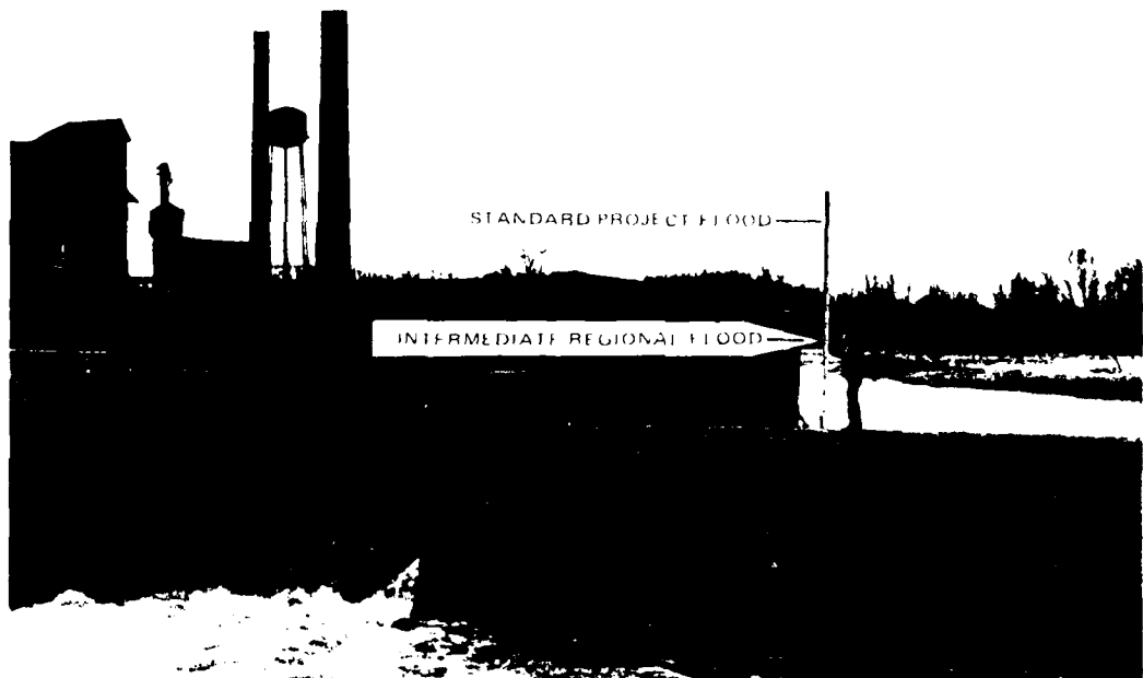
Figure 14 - Future flood heights at Wheatland Center Road dam near General Aniline & Film Corporation facility. Photo taken January 1973.
