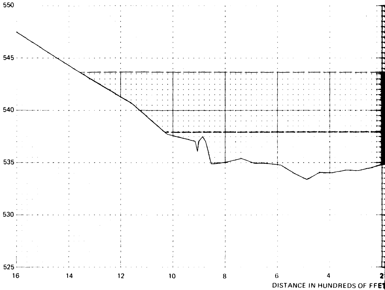
CROSS SECTION NO. 24 MILE POI
