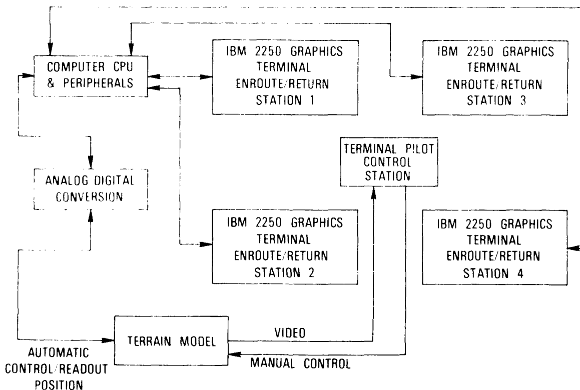
Figure 1. HUMAN ENGINEERING SYSTEMS SIMULATOR FACILITY CONFIGURATION
