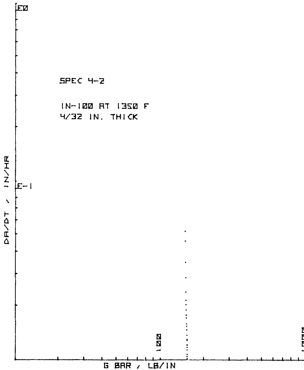
Figure 222. da/dt vs. \bar{G} for Ring Specimen 4-2
