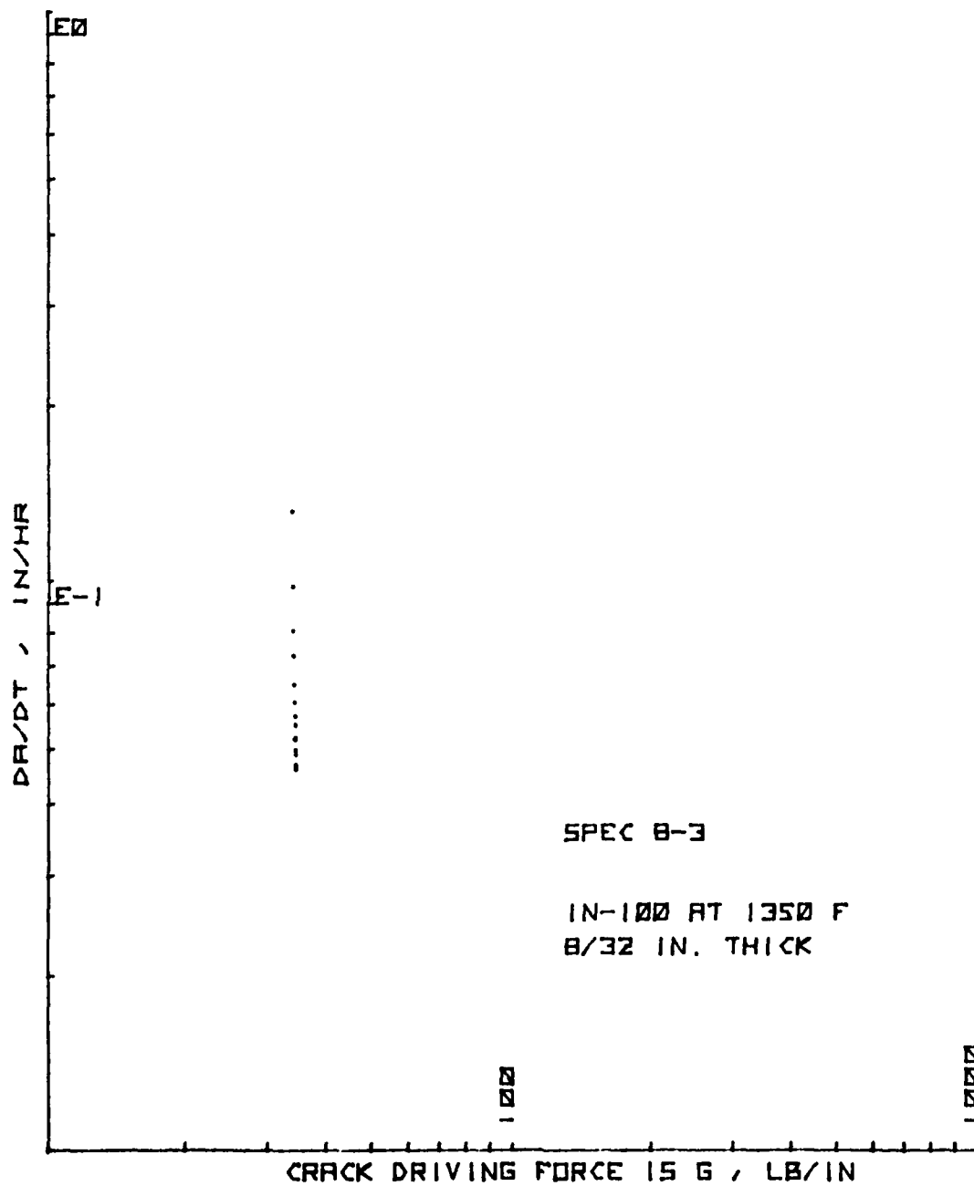
Figure 218. da/dt vs. G for Ring Specimen 8-3
