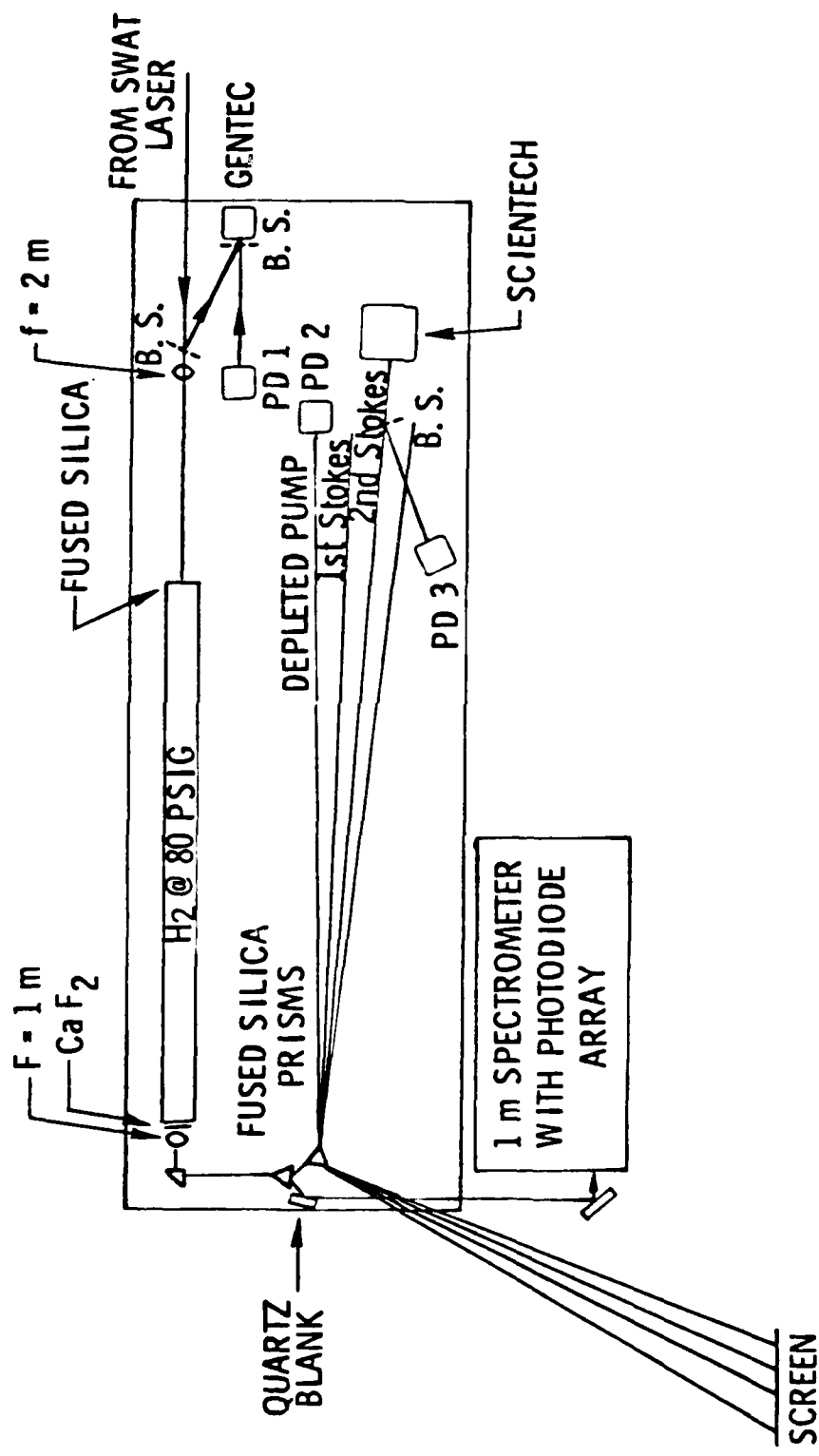
Figure 6. Setup for Raman Oscillator Experiments
