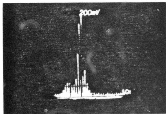
(b) INJECTION-LOCKED XeF LASER SPECTRUM (INSTRUMENT LIMITED RESOLUTION \approx .4 \text{ Å FWHM} )
