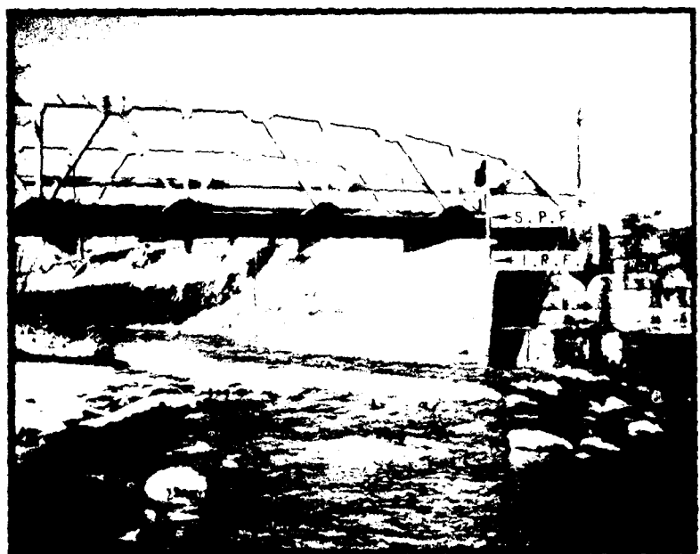
Figure 24 - Arrows indicate the heights of the Standard Project and Intermediate Regional Floods at Noff Road bridge, stream mile 33.42. Photo taken March 1971.
