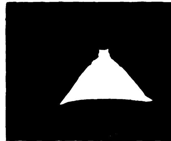
NSC/E2, filled notch C/M = 0.23
