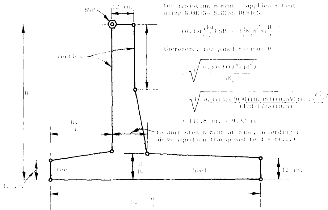
Figure 3-6. Wall cross section with illustration of all default values for hydraulic structures (default values are taken from EM 1110-2-2501, unless otherwise noted)
