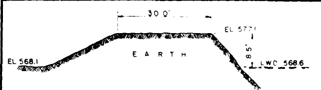
SECTION OF SQUAW ISLAND DIKE BUILT 1822, 1825, 1922, 1923
