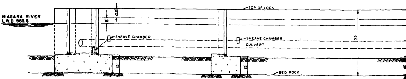
PROFILE BLACK ROCK SHIP LOCK NOT TO SCALE
