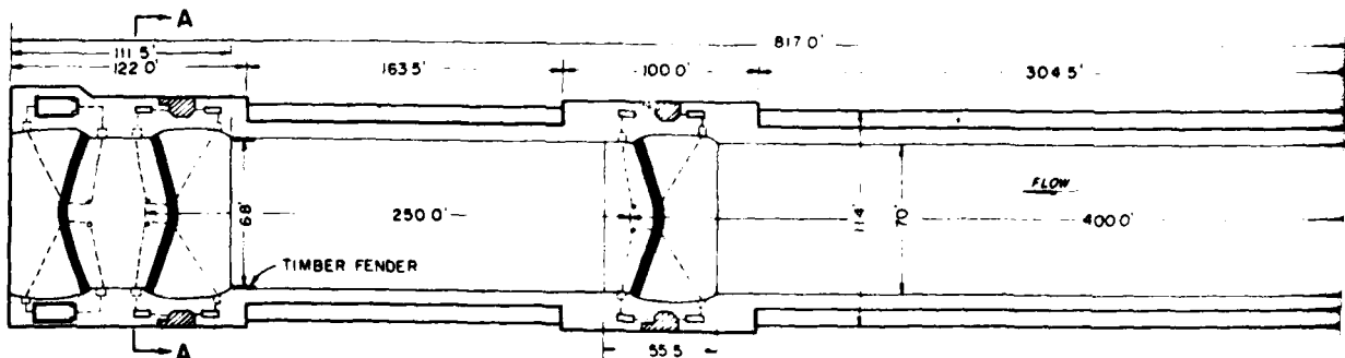
PLAN OF BLACK ROCK SHIP LOCK NOT TO SCALE
