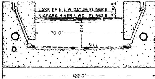
SECTION OF LOWER GATE SPACE AT A-A
