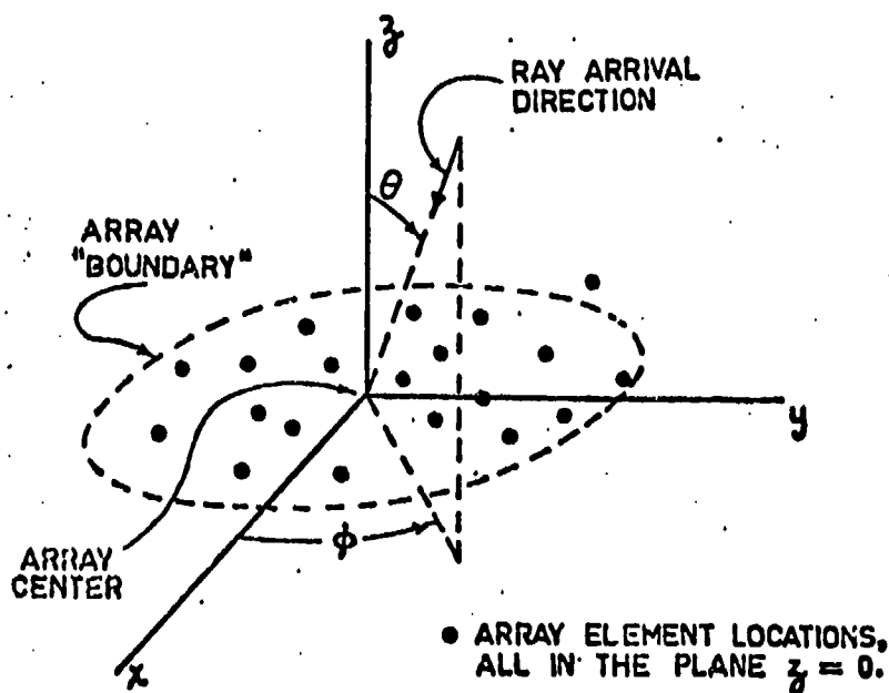
FIGURE 1. ARRAY GEOMETRY
