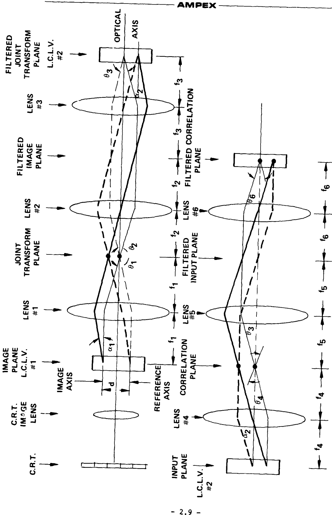
Figure 2.5 JTC Optical Schematic
