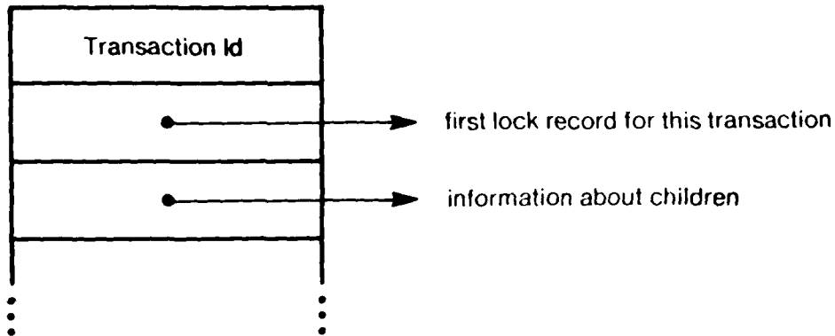
Transaction Record Format
