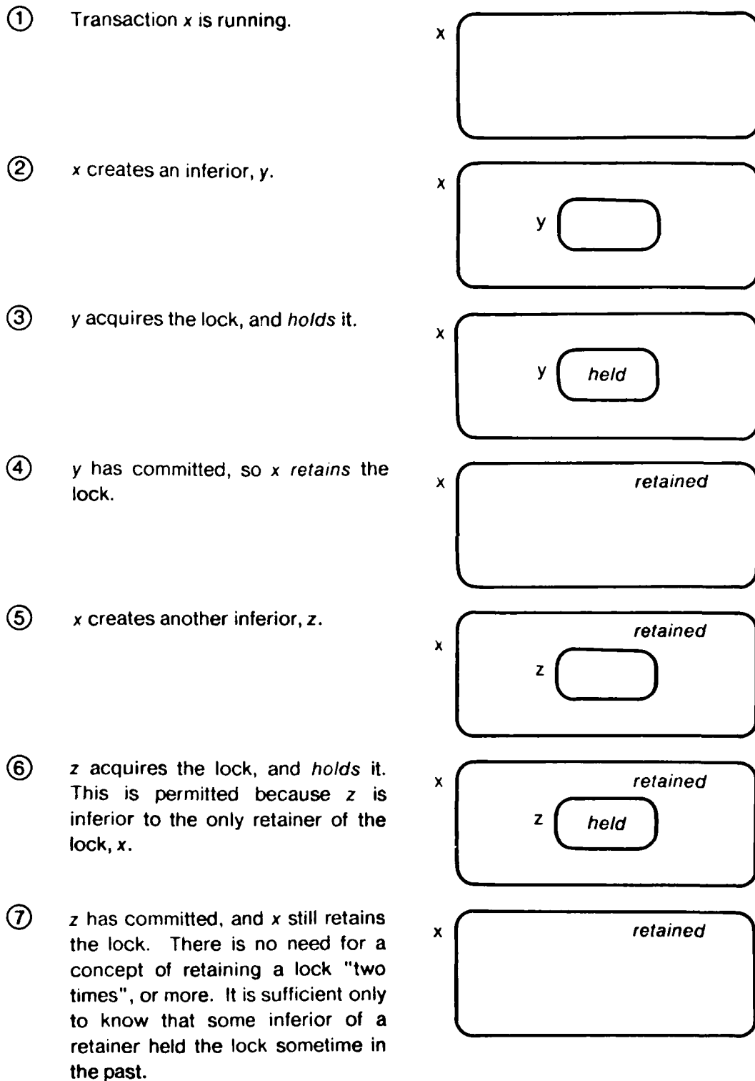
Figure 1. Example of Lock Inheritance.
