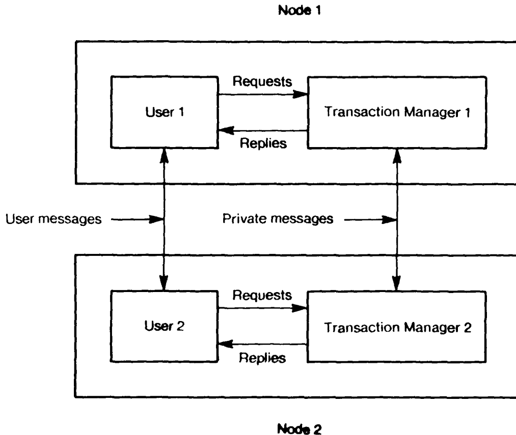
Figure 3. Transaction Manager Relationships.
