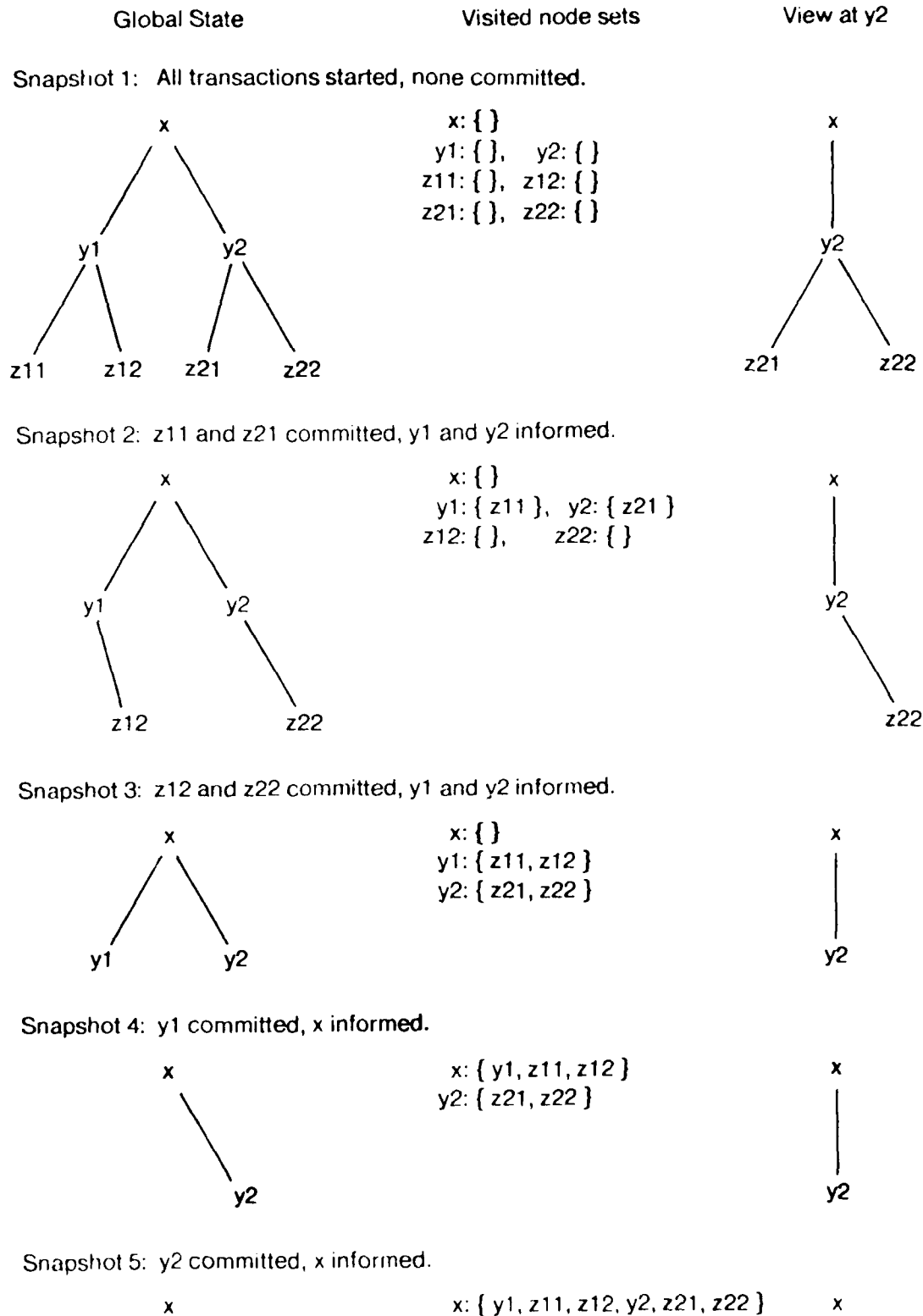
Figure 4. Example of Commitment.
