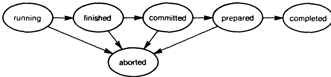
Top-Level Transaction State Diagram
