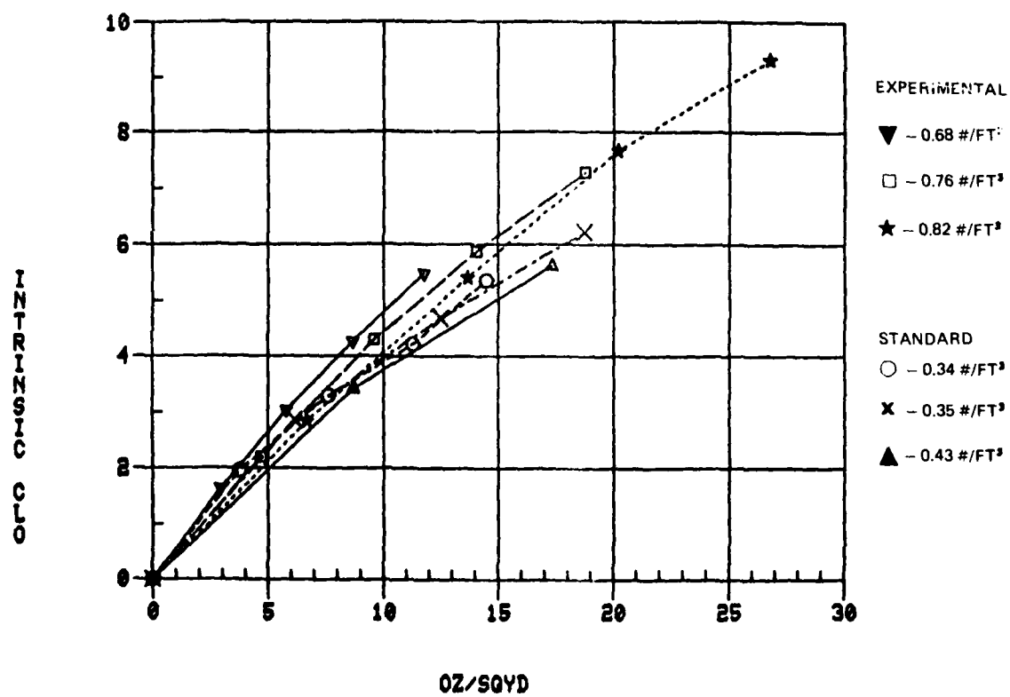
Figure 6. Experimental & Standard Batting - Thermal Resistance vs. Areal Density
