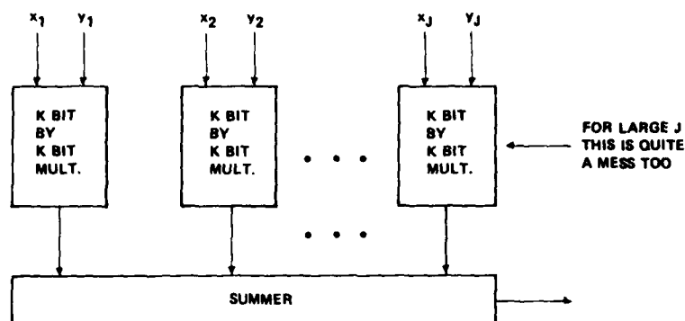
Figure 5 Conventional Mechanization
