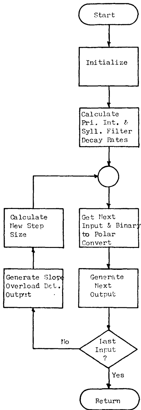
Figure 7. CVSD Decoder Subroutine Flowchart
