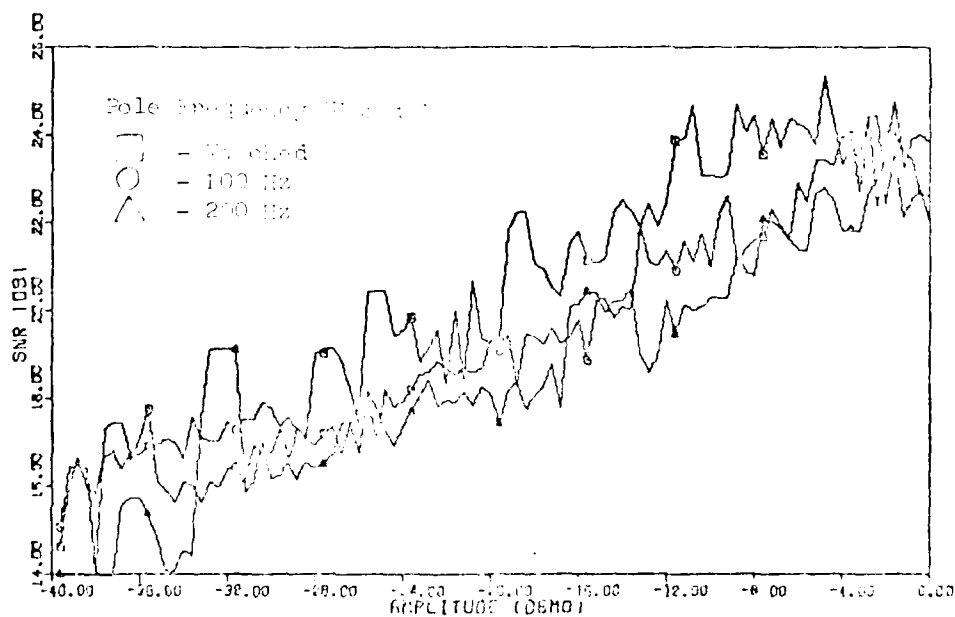
Figure 4.8b. CVSD System Signal-to-Noise Performance vs. Input Signal Power with Encoder and Decoder. Primary Integrator Pole Frequencies Mismatched at 32 kb/s Baud Rate. (100 Hz Test Bit Rate).
