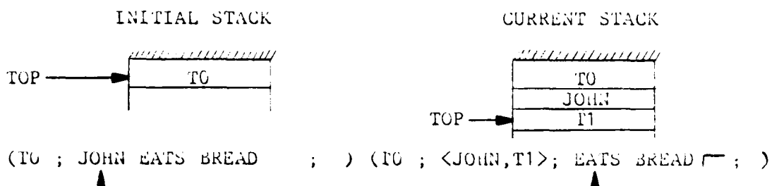
Figure 3-2: Result of the 'Shift, T1' move
