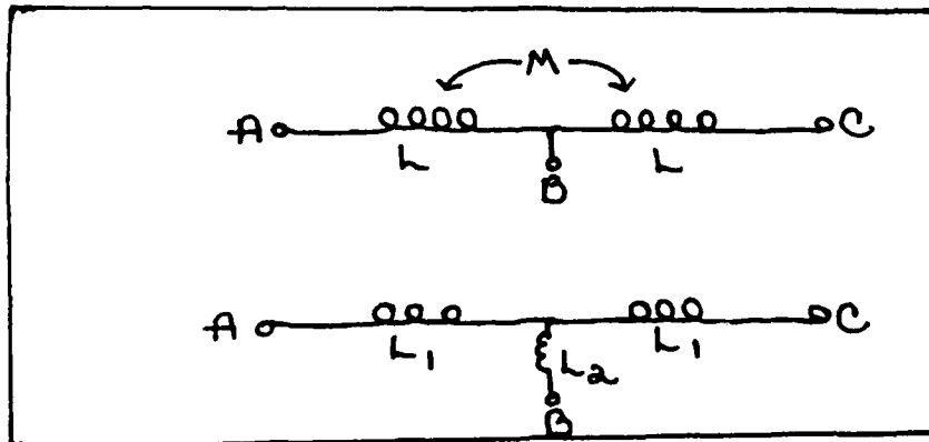
Figure 27. T Equivalent Circuit of Two Series Coils
