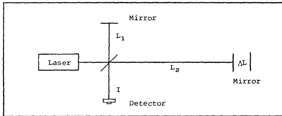
Figure 2.1 Michelson Interferometer
