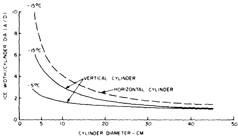
FIG. 7(b): EFFECT OF CYLINDER DIAMETER ON ICE WIDTH
