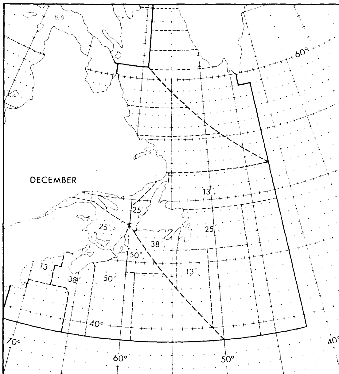
FIG. 24: PERCENTAGE OF YEARS FOR WHICH ICING OF SEVERITY GREATER THAN SLIGHT HAS BEEN REPORTED IN THE VARIOUS ICNAF DIVISIONS FOR THE MONTH OF DECEMBER
