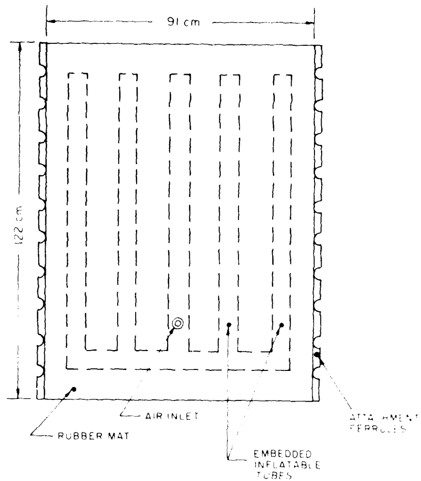
(a) LAYOUT OF PNEUMATIC DE-ICER
