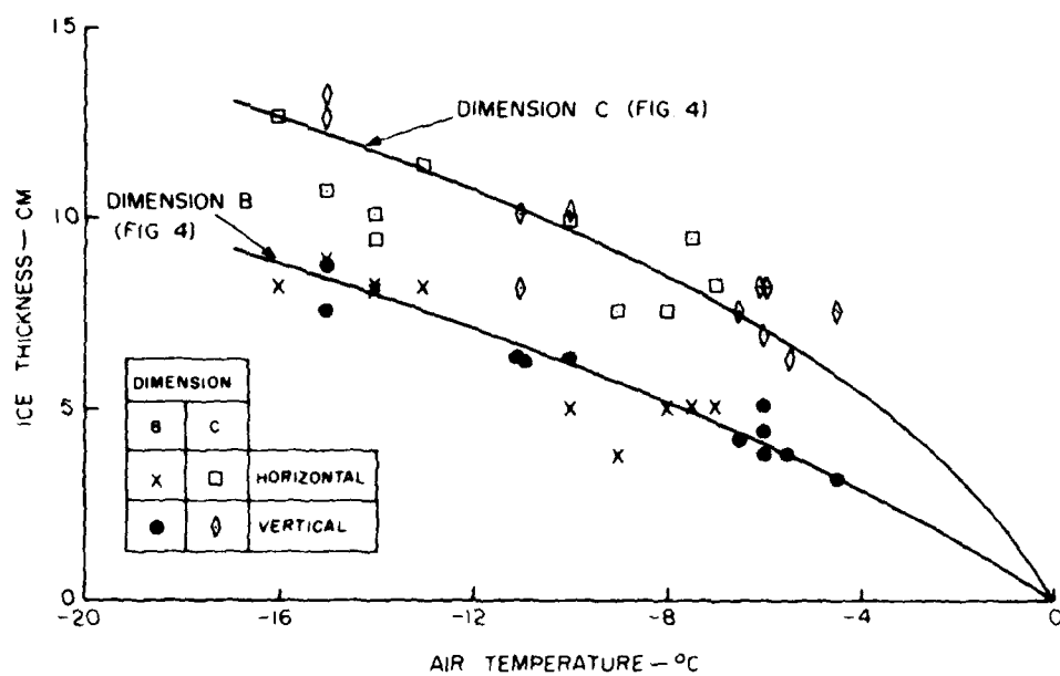
FIG. 7(a): EFFECT OF TEMPERATURE ON ICE THICKNESS
