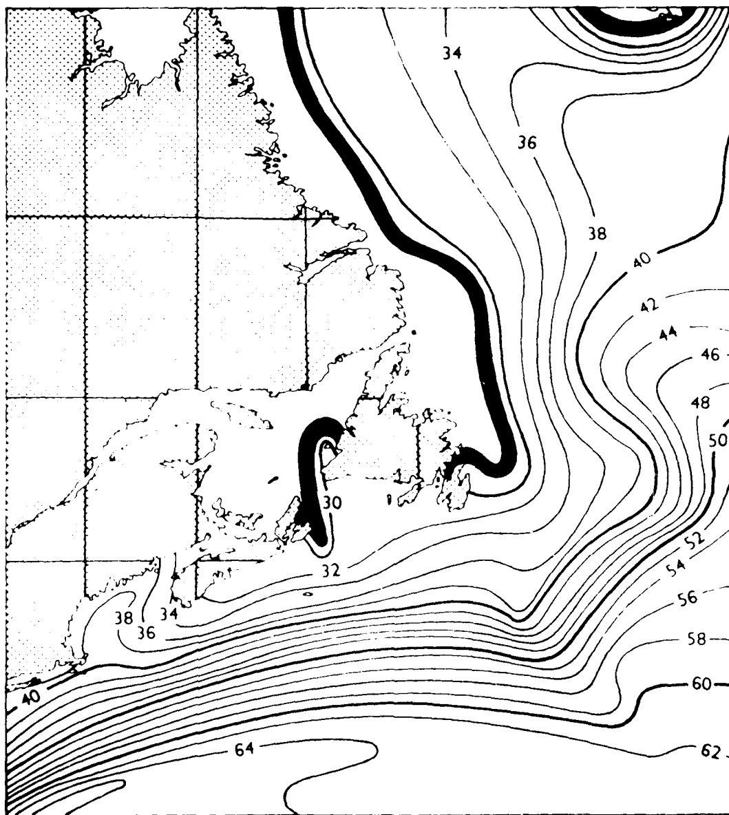
FIG. 17: MEAN SEA-SURFACE TEMPERATURE (°F) FOR FEBRUARY (FROM OCEANOGRAPHIC ATLAS - REF. 37)
