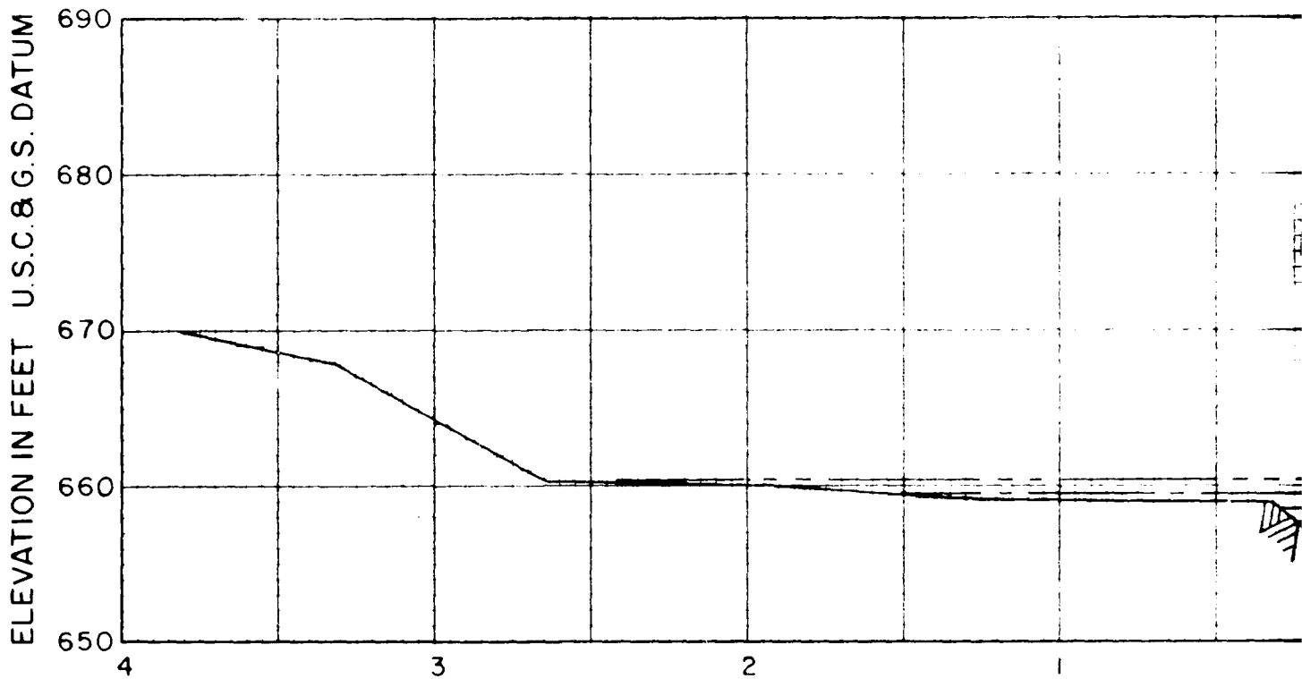
PENITENTIARY GLEN CREEK CROSS SECTION NO. 27
