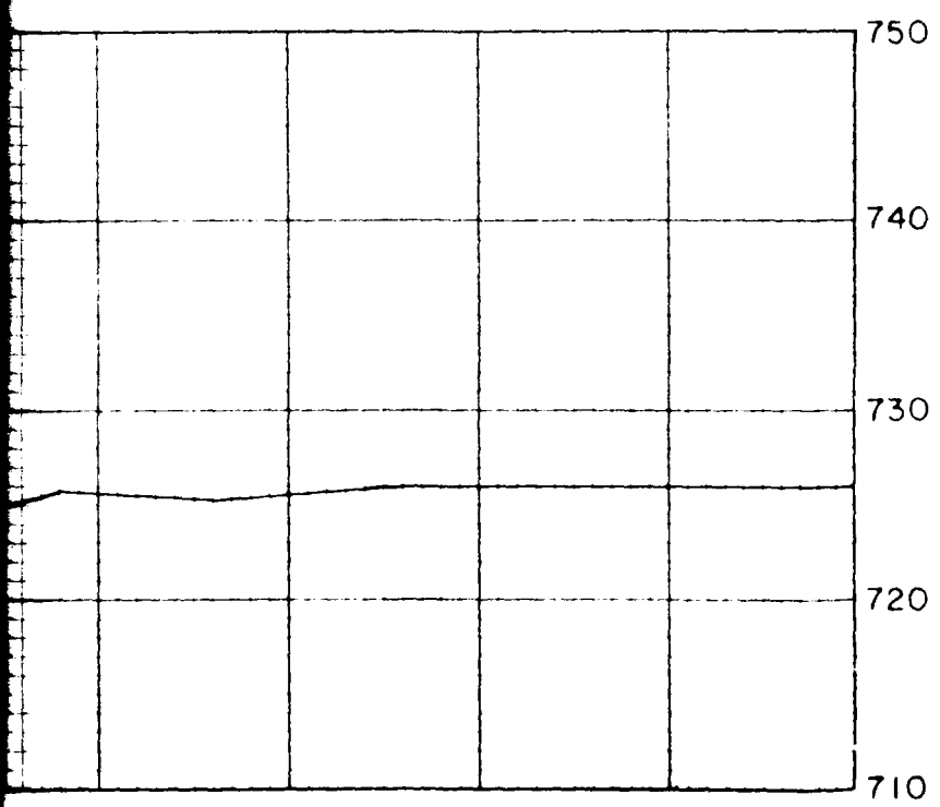
STATION NO. 31 MILE POINT 0.85
