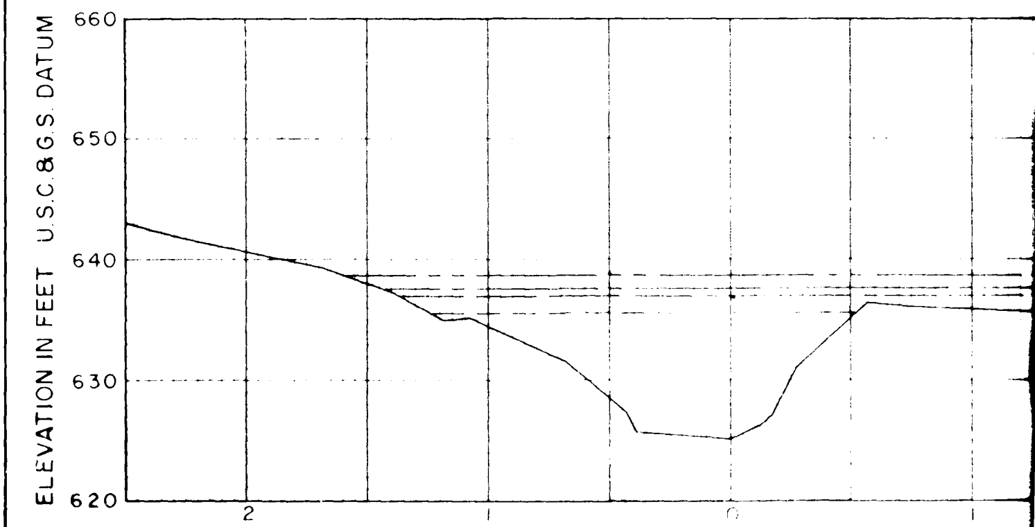
DISTANCE IN HUNDRE CROSS SECTION NO. 5
