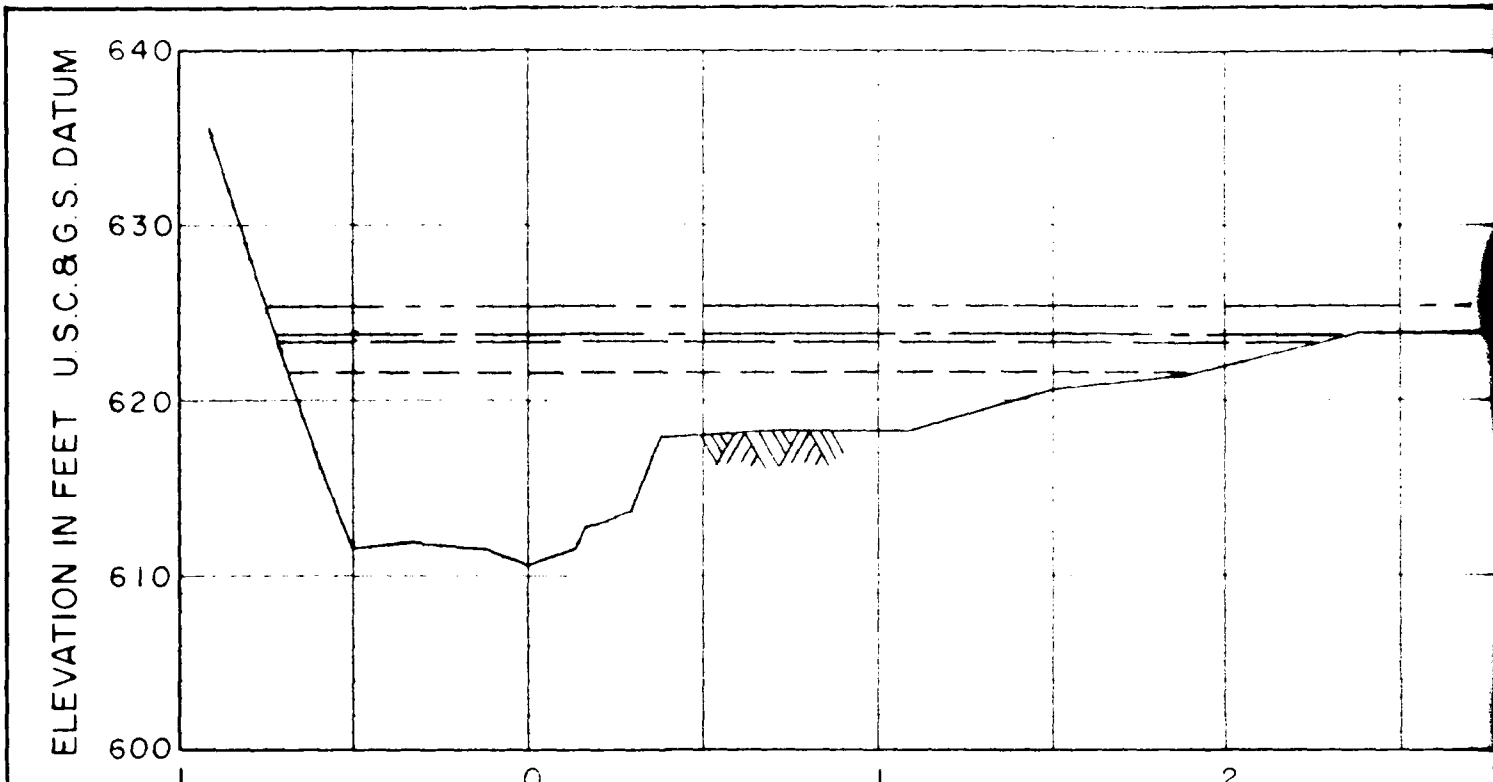
DISTANCE IN HUNDRE CROSS SECTION NO. 3
