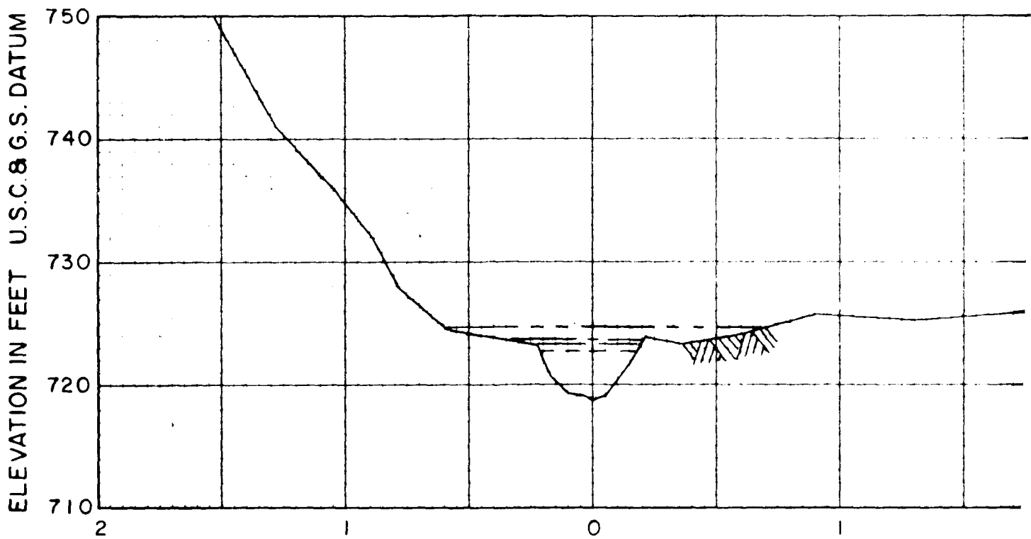
PIERSON CREEK CROSS SECTION NO. 31
