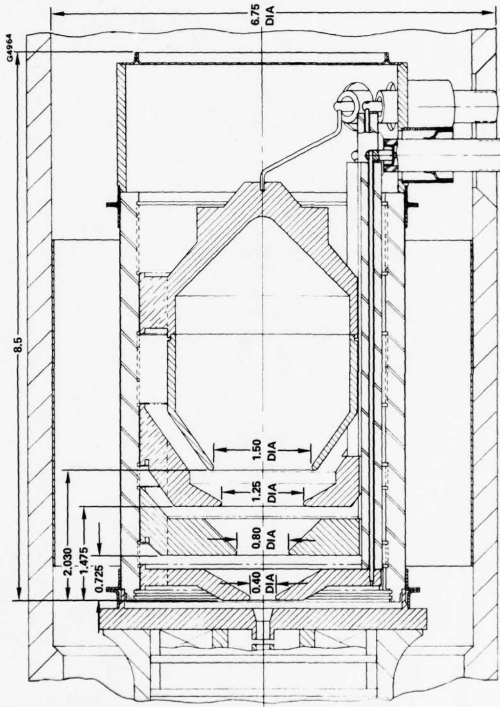
Figure 17 Schematic layout of four-stage depressed collector for 673H. Dimensions are in inches.
