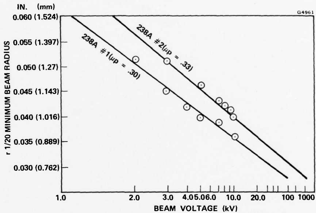
Figure 7 238A demountable guns V_b vs r \ 1/20 .
