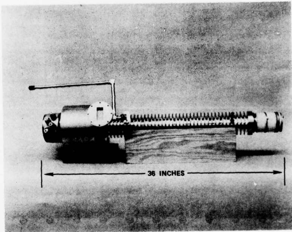
Figure 23 Completed 673H tube ready for processing.
