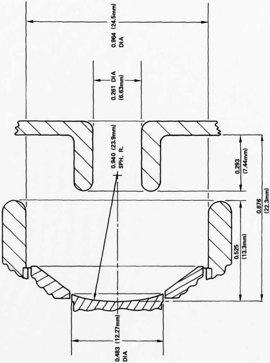
Figure 9 Electron gun dimensions.
