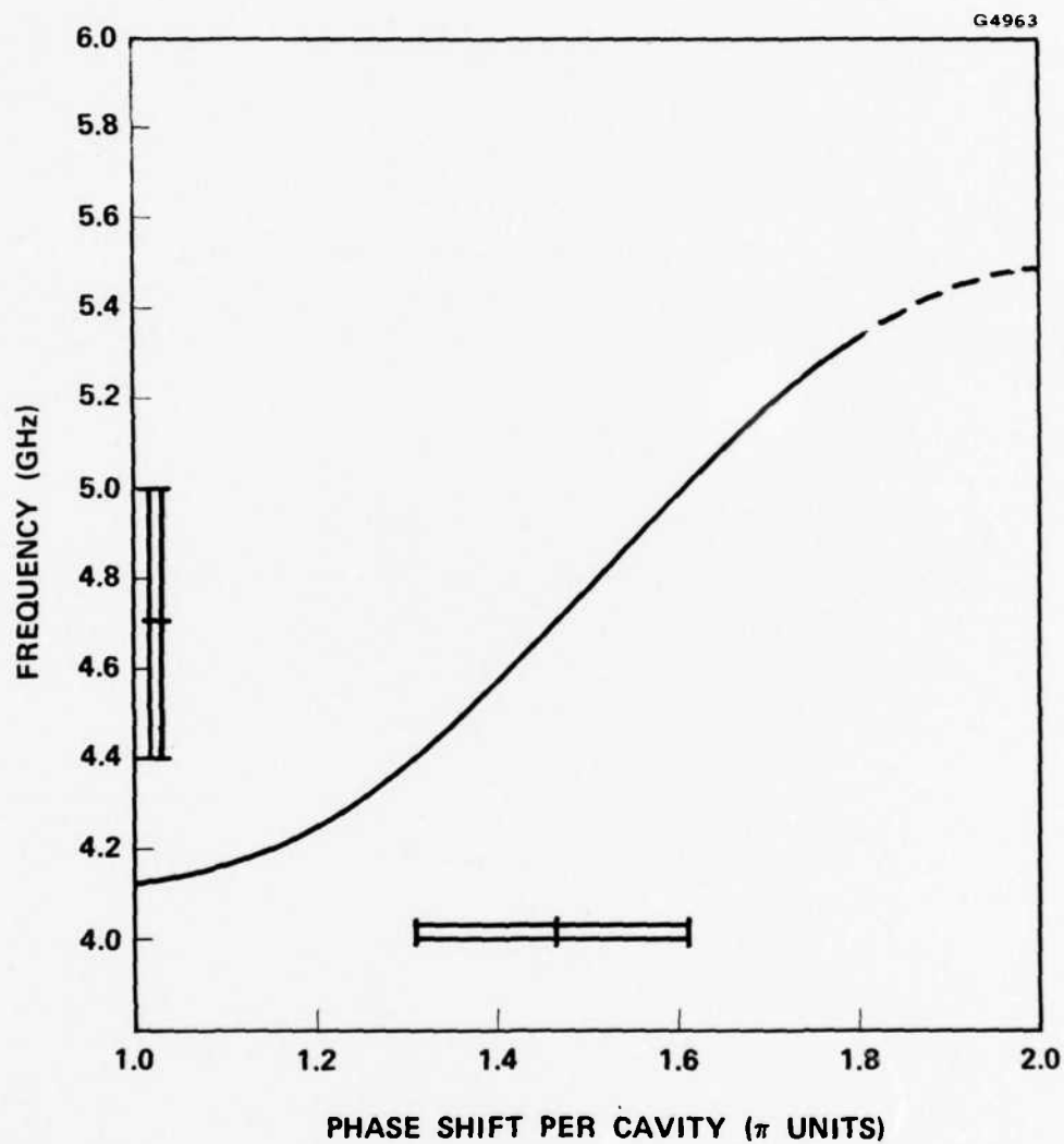
Figure 14 Measured frequency vs phase ( \omega\beta ) characteristic of interaction circuit.
