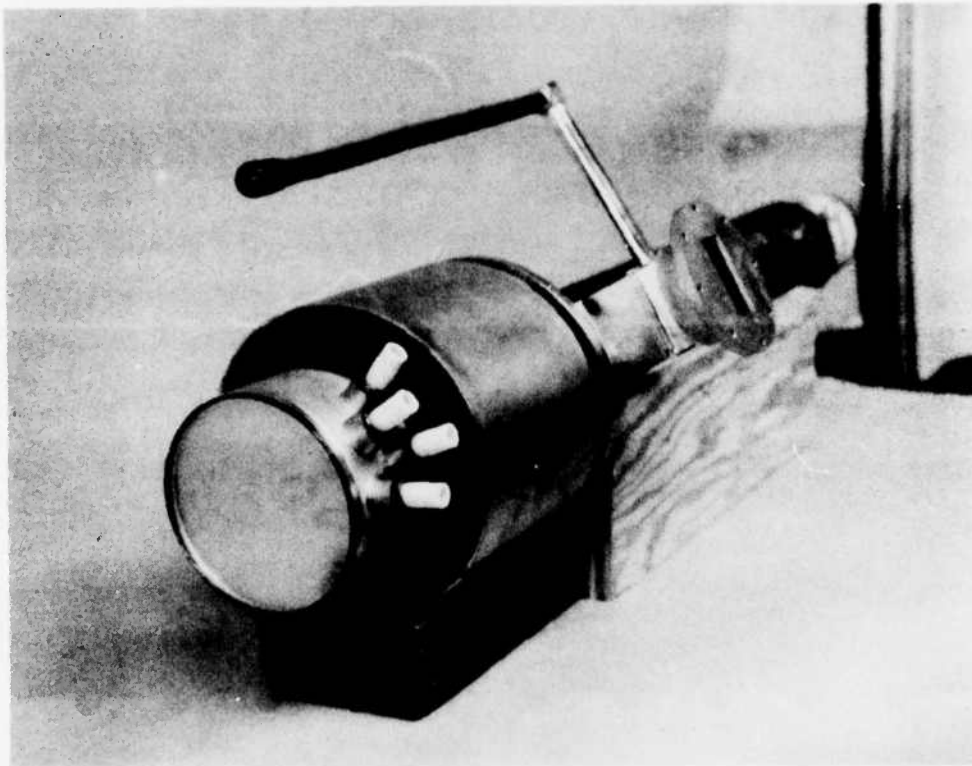
Figure 24 End view of 673H showing details of collector cooling fins and high voltage feedthroughs.
