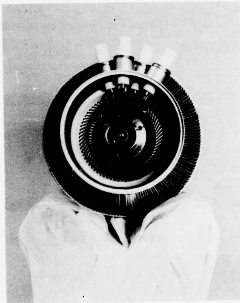
Figure 22 End view of completed 4-stage collector assembly.
