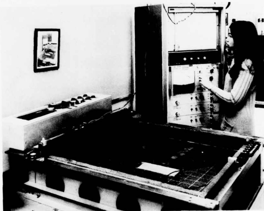
Figure 1 Electrolytic tank.
