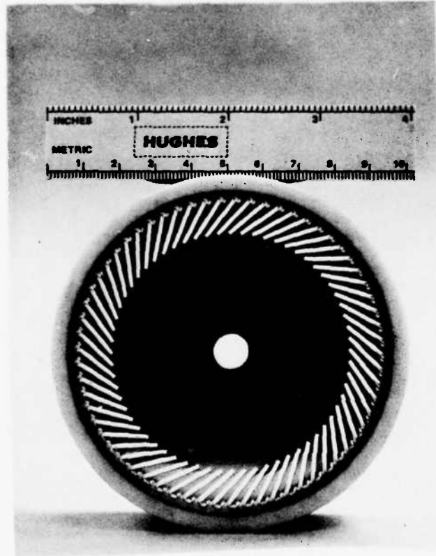
Figure 18 673H simulated collector electrode to ceramic brazed assembly.
