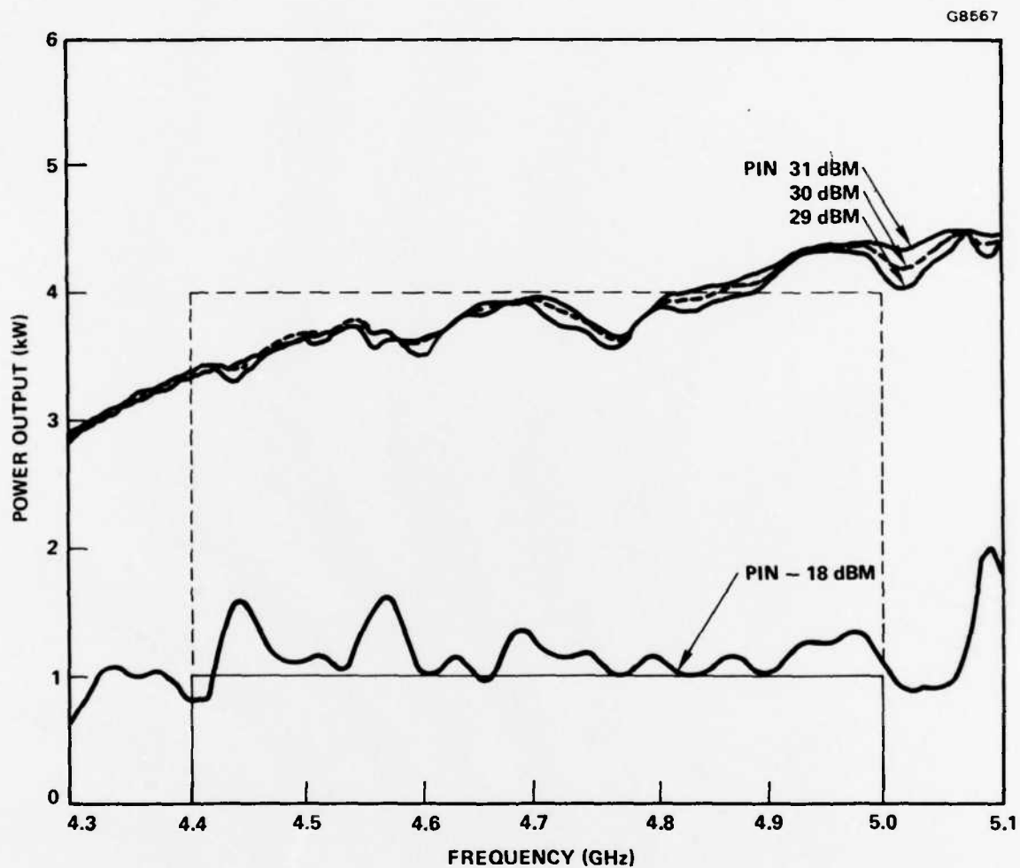
Figure 25 Power output versus frequency of 673H at -24 kV cathode voltage.
