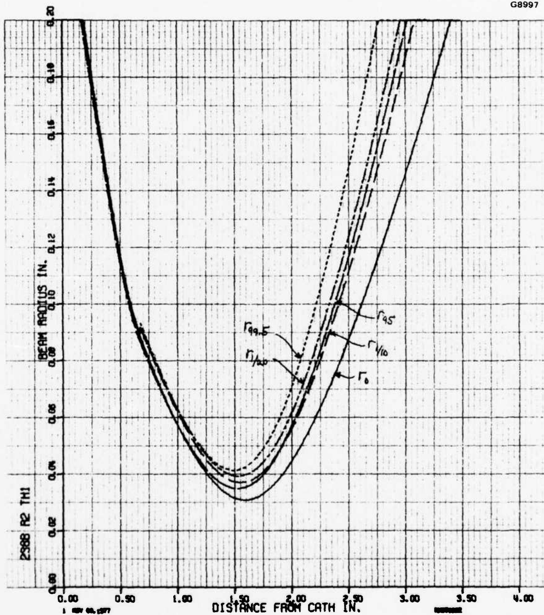
Figure 4 Computed electrostatic beam envelopes of 238B gun.
