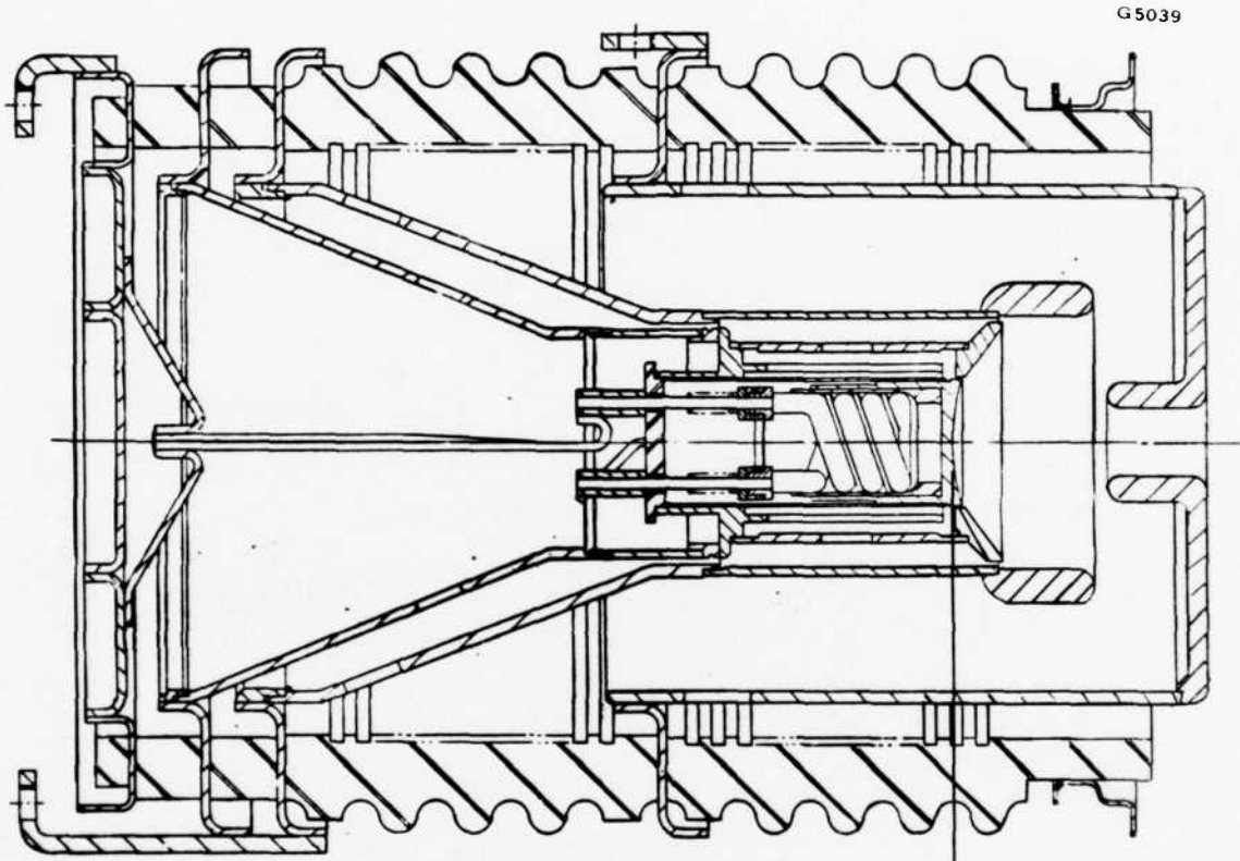
Figure 8 238B isolated anode electron gun.
