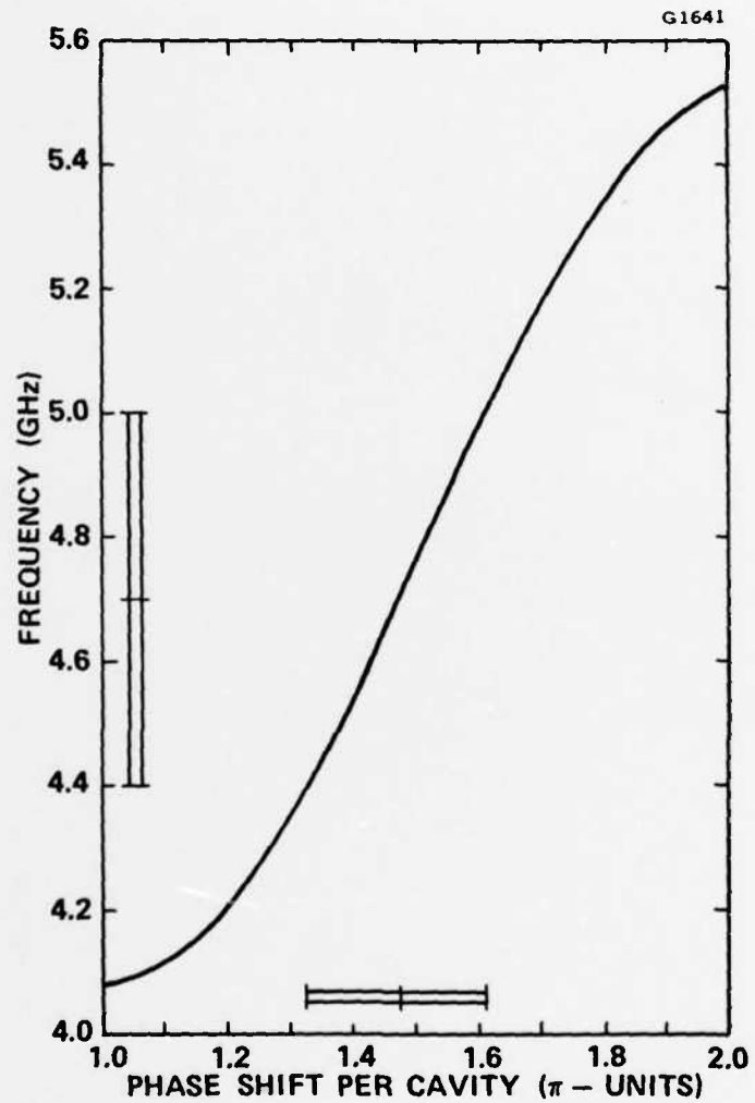
Figure 10 Theoretical frequency-vs-phase ( \omega\beta ) characteristic of interaction circuit.
