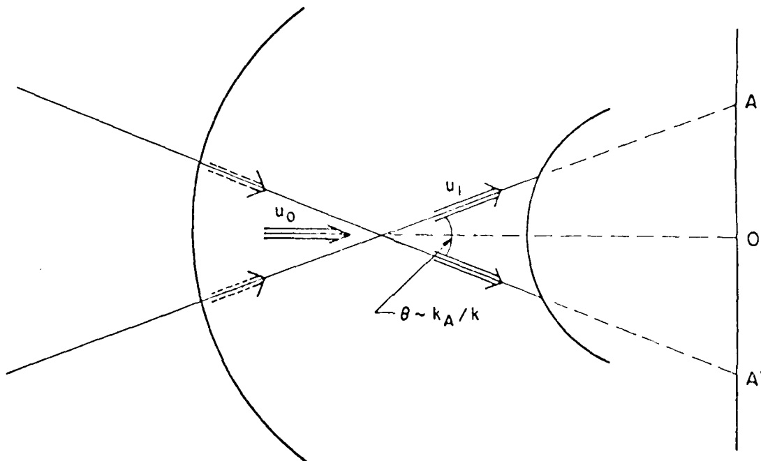
Figure B-1. Illustration of the Reproducibility of the Scattered Wave. The unperturbed wave focuses (virtually) at the point O in the common focal plane of the two mirrors. The scattered waves also focus in this plane but at slightly displaced points A and A' . The return waves after one round trip will then be in the same direction as the original scattered waves.
