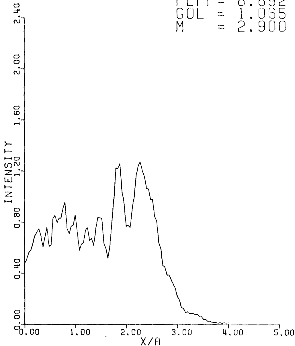
Figure 22. Intensity Profile for G_0L = 1.065 , F_{eff} = 8.892 . The result here is very similar in detail to the empty resonator case (Figure 19) but the envelope of the distribution is flatter.
