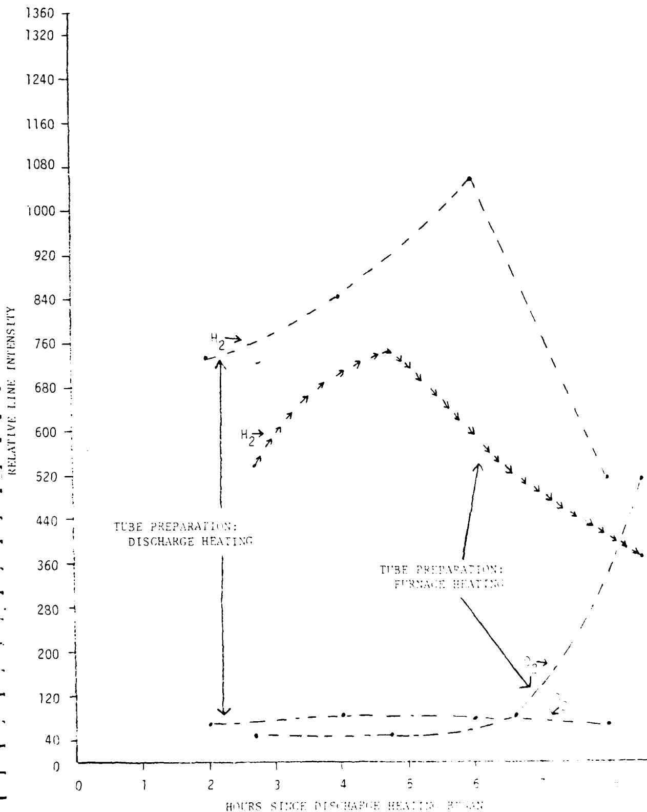
FIGURE 12. COMPARISON OF HYDROGEN 4314 \text{\AA} AND OXYGEN 5331 \text{\AA} LINE INTENSITY DURING STANDARD LEAD LASER RUN. TUBES PREPARED BY FURNACE HEATING OR DISCHARGE HEATING.
