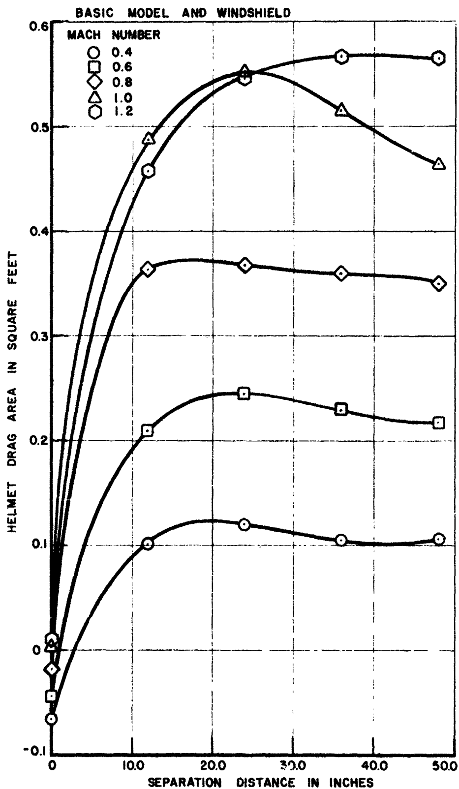
Figure S2. The effect of separation distance on helmet drag, for the basic model and windshield, without flow diverter. Yaw = 0.0^\circ . Pitch = 5.0^\circ .
