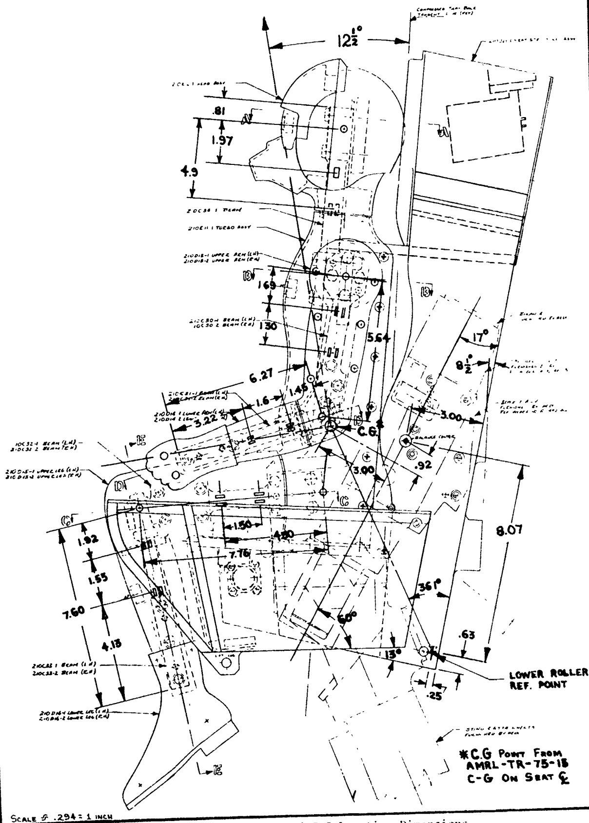
Figure 6. Strain gauge and C-G Locating Dimensions
