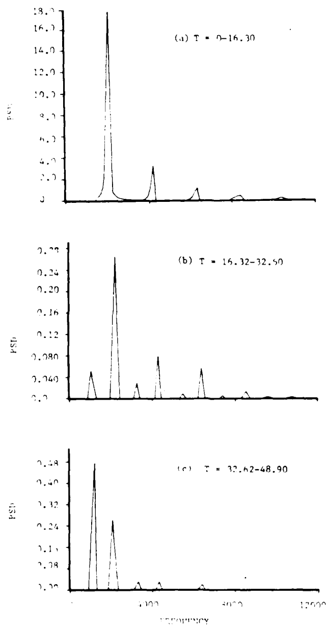
Figure 21 (a), through (c). Time Evolution of Power Spectral Density as a Function of Frequency, for a Standing Pulse, \langle P \rangle = 0.4 \text{ mW/cm}^2 , \lambda = 0.63 \mu\text{m} , \text{ACM} = 1 .
