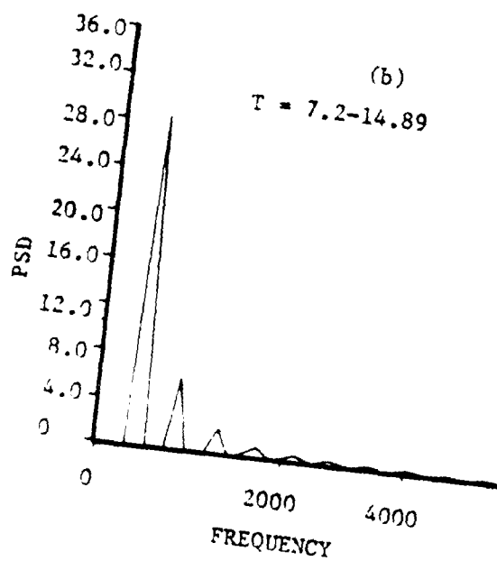
Figure 9(b) and (c). Time Evolution of PSD as a Function of Frequency Utilizing Hyman's Scheme with \beta = 0.3 .
