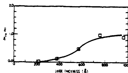
Figure 7. \Delta V_{FB} as a function of oxide thickness for as-grown oxides following 0.5 M rad \text{Co}^{60} irradiation at room temperature and at applied field of 1 MV/cm (from Ref. 51).
