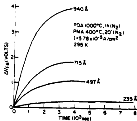
Figure 5. \Delta V_{FB} as a function of time for various oxide thicknesses for avalanche injection of electrons (from Ref. 44).
