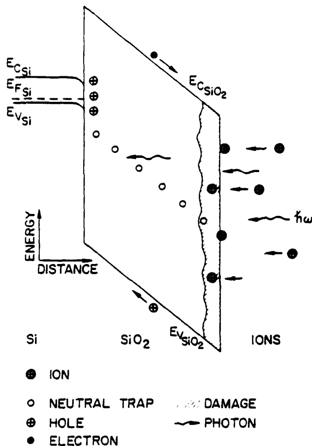
Fig. 1 Energy band diagram for thermal \text{SiO}_2 layer on an underlying silicon substrate exposed to low-energy positive ions and photons which are present in an RIE reactor.
