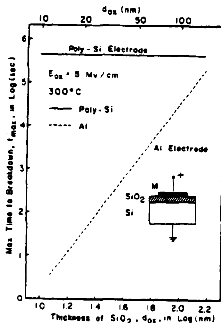
Figure 4. Maximum time to breakdown vs. thickness of \text{SiO}_2 with Al and Si electrodes in MOS capacitors (from Ref. 2).
