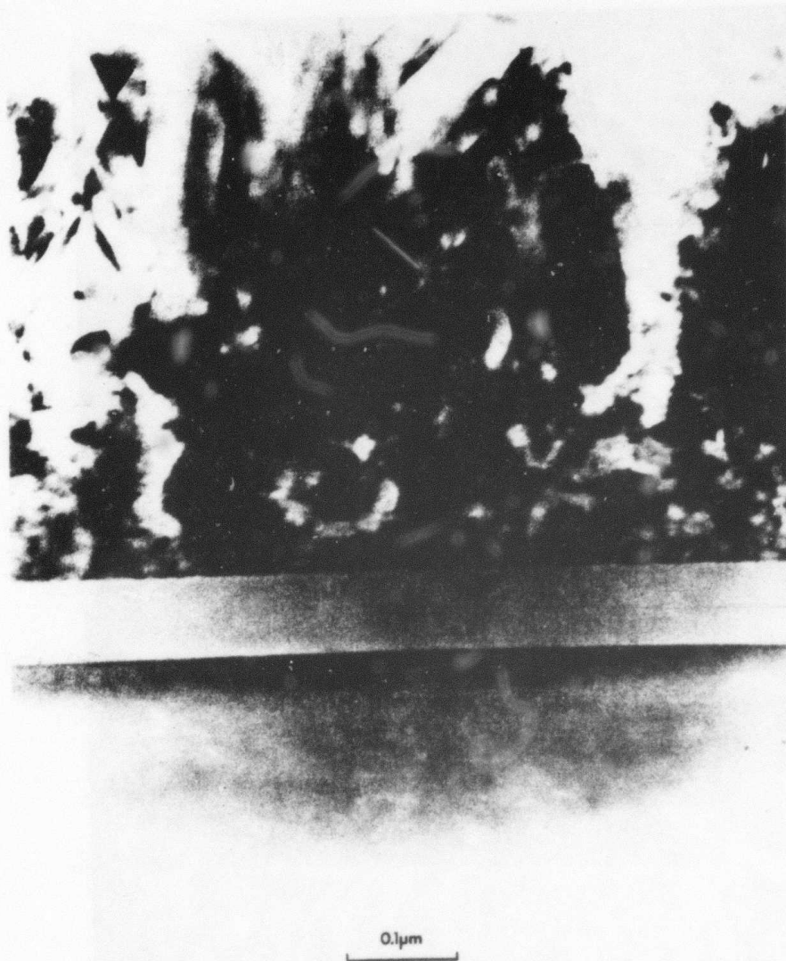
Figure 4. Bright-field cross-section TEM of the top part of the Si substrate, thermal gate \text{SiO}_2 layer, and the lower part of the first poly-Si layer (floating storage layer). Poly-Si layers are undoped.
