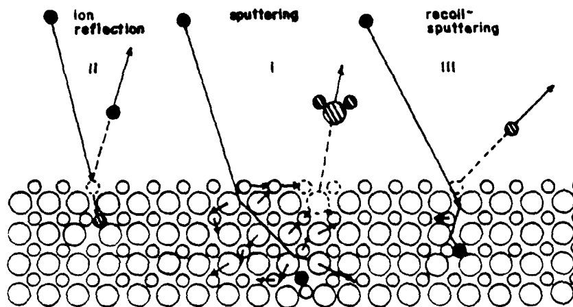
Figure 4-1 Interaction processes of an ion with a solid surface resulting in the emission of heavy particles. (ref. 3).
