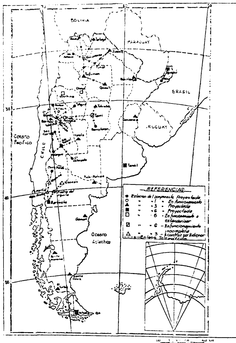
FIGURE II-1 NATIONAL SEISMIC NETWORK OF THE REPUBLIC OF ARGENTINA (INPRES, 1979)
