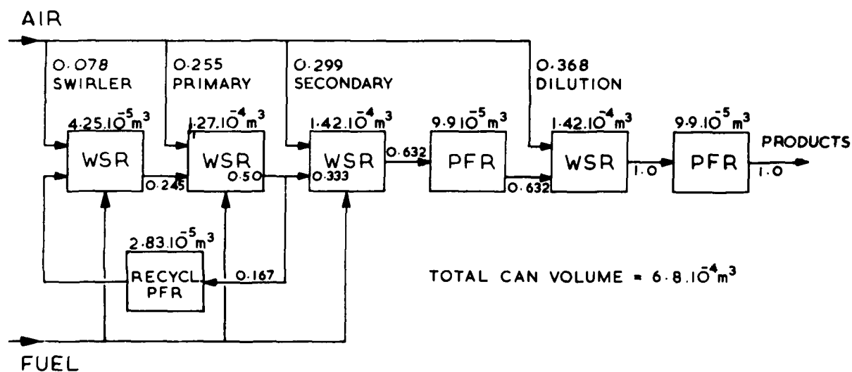
FIGURE 2. Recycle loop diagram.
