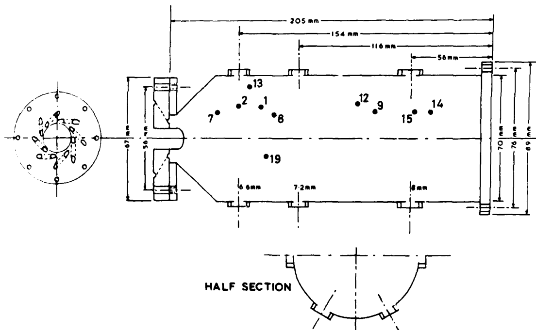
Figure 9. Reactor with 1.84 liter liquid volume and 1.5 liter gas volume.
