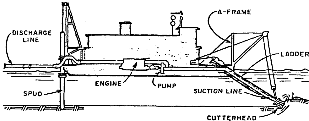
Fig. 6.2. Pipeline Dredge.
