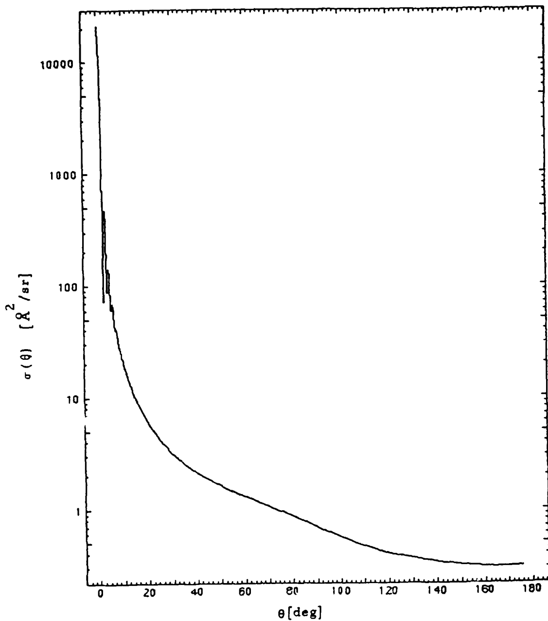
Fig. 12. Semilog plot of the He-0 differential cross section \sigma(\theta) as a function of the scattering angle \theta for E = 1.66 eV
