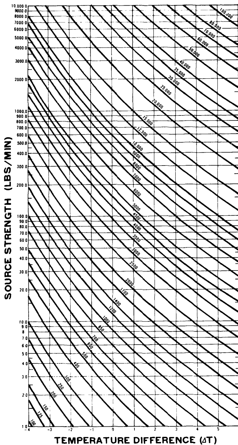
Figure 4. Nomogram for Determining Diffusion Factors (DF). DF = 0.513 (\Delta T + 30)^{2.53} . The DF values are indicated by the curved diagonal lines as labeled.
