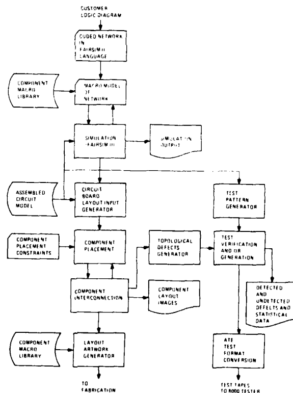
Figure 3 Fairchild System Flow Diagram
