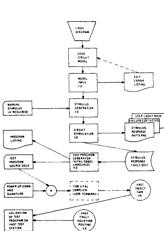
Figure 1 LASAR II System Flow Diagram
