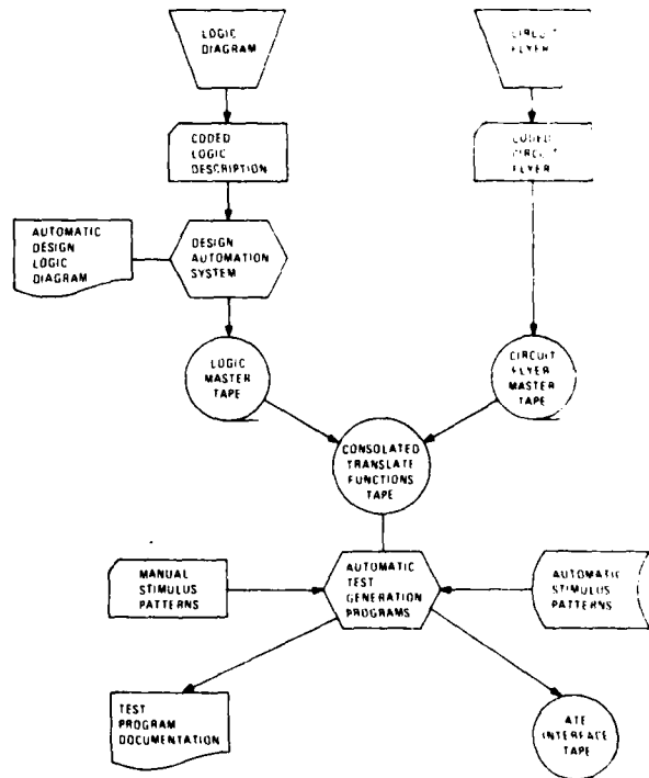
Figure 11 SALT System Flow Diagram
