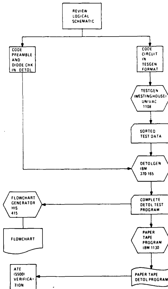
Figure 7 CAD System Flow Diagram
