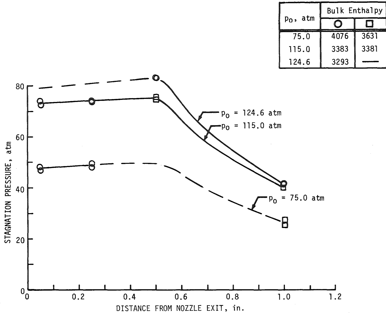
Figure 23. Centerline axial pressure distribution for M = 2.0 , d^* = 0.625 in., d_e = 0.850 in., and I = 950 amp.
