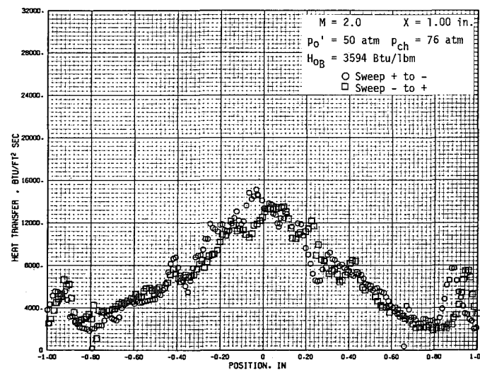
Figure 24. Radial heat-transfer profiles using a calorimeter with R_N = 0.25 \text{ in.} , M = 2.00 , d^* = 0.625 \text{ in.} , d_e = 0.850 \text{ in.} , and I = 950 \text{ amp.}
