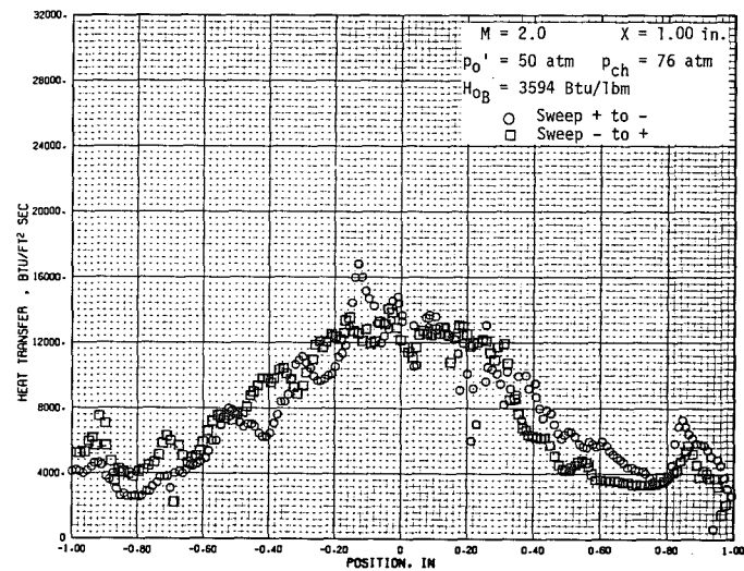
Figure 25. Radial heat-transfer profiles using a calorimeter with R_N = 0.15 in., M = 2.0 , d^* = 0.625 in., d_e = 0.850 in., and I = 950 amp.
