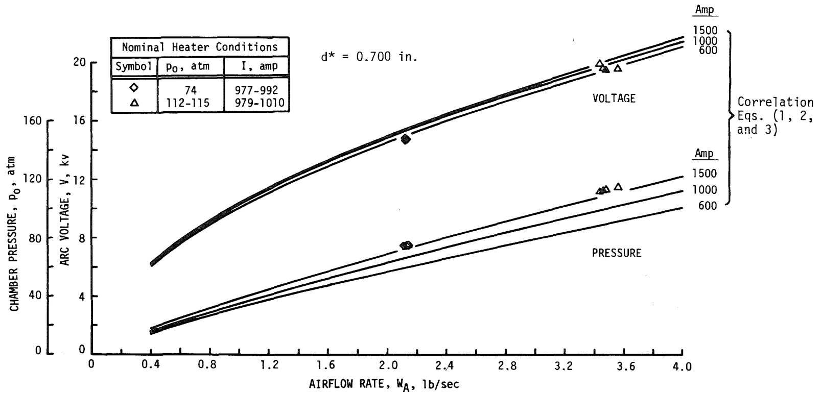
Figure 19. Heater pressure and voltage for d^* = 0.700 \text{ in.}
