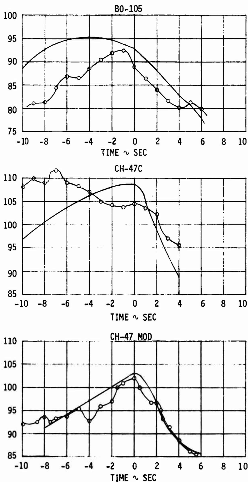
FIGURE 1. COMPARISON OF PREDICTED AND MEASURED PNL TIME HISTORIES - FLYOVER
