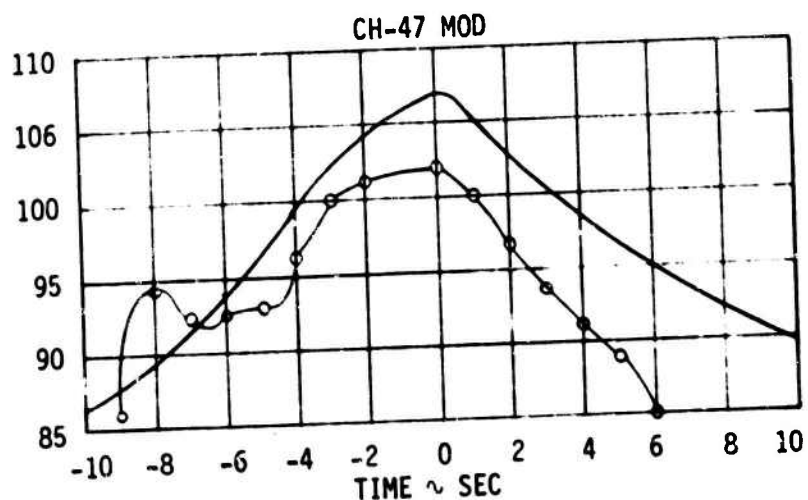
FIGURE 3. COMPARISON OF PREDICTED AND MEASURED PNLT TIME HISTORIES - TAKEOFF
