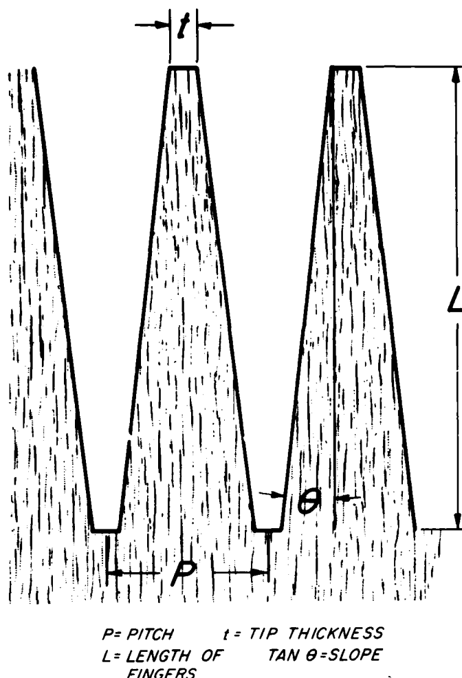
Figure 2.—Finger joint and identifying nomenclature.
