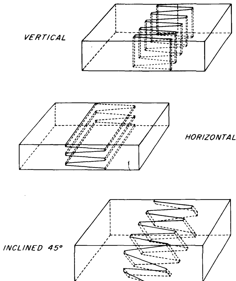
Figure 3.—Orientations of finger joints.
