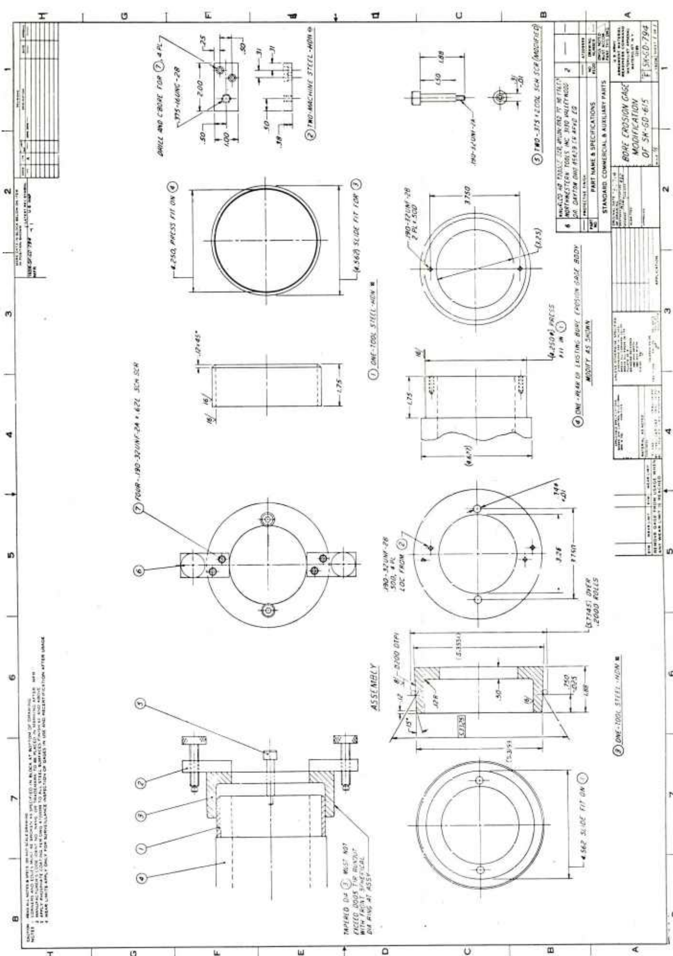
Figure 4. Detail description of modification assembly.
