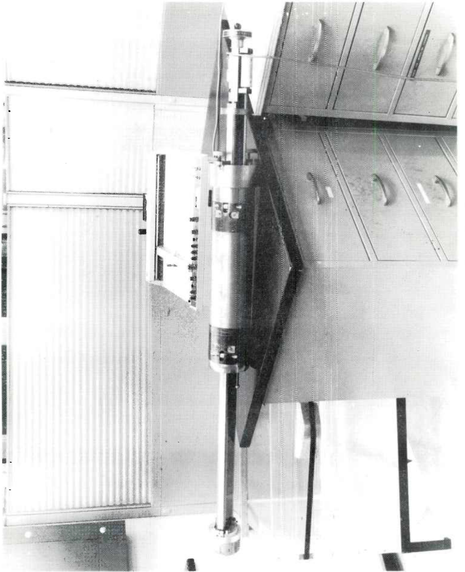
Figure 1. Bore erosion measuring system.
