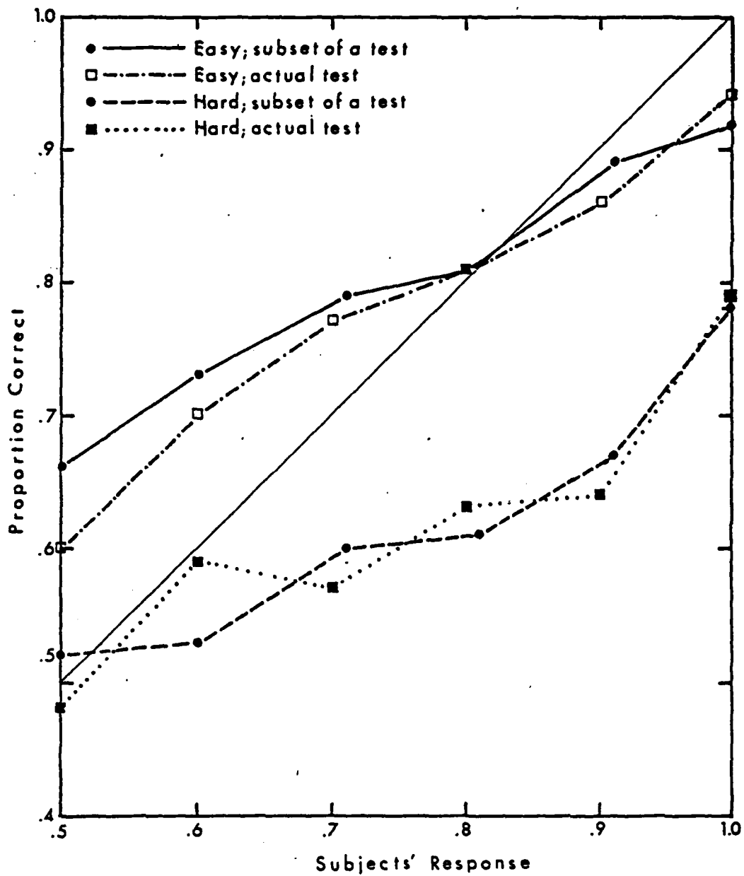
Figure 3. Calibration for hard and easy tests and for hard and easy subsets of a test.
