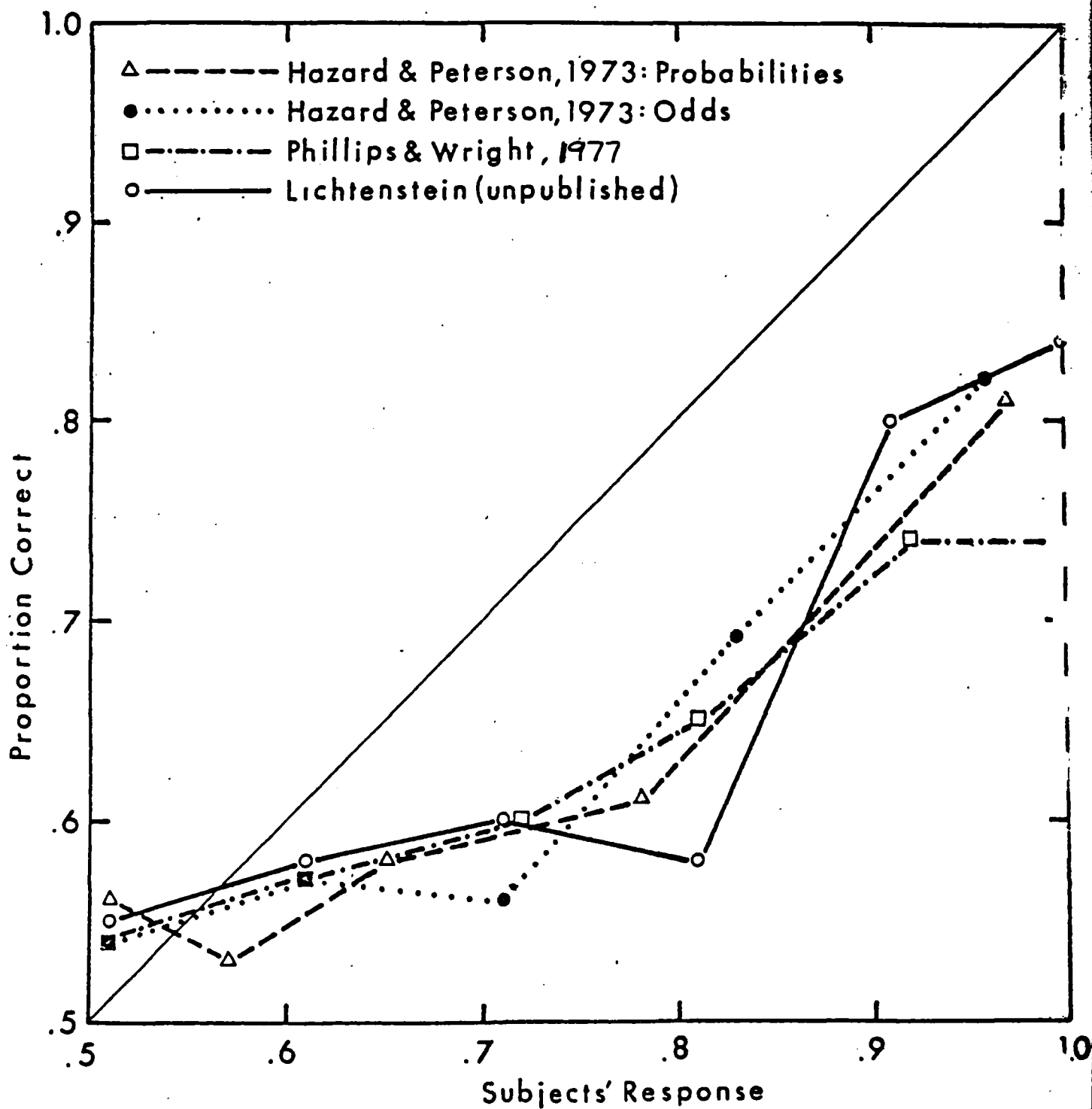
Figure 2. Calibration for half-range, general knowledge items
