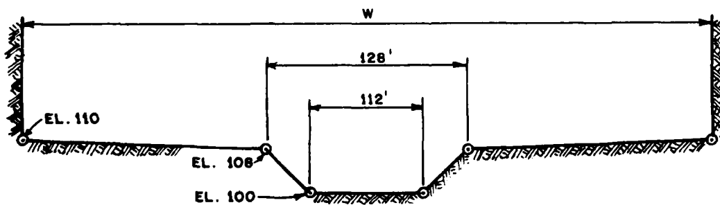
FIGURE 3.2 River Cross Section Used in Analysis
