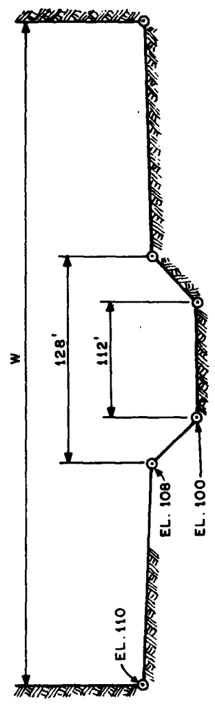
RIVER CROSS SECTION USED IN ANALYSIS
