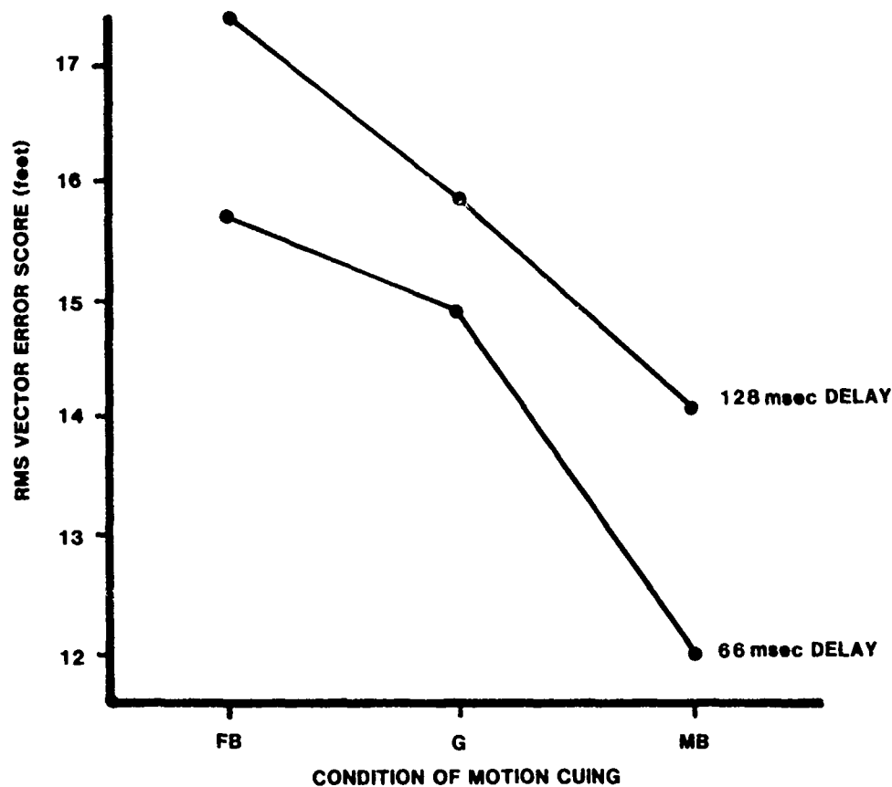
Figure 13. Vector Error Score Averaged Over Conditions of Ship Motion.
