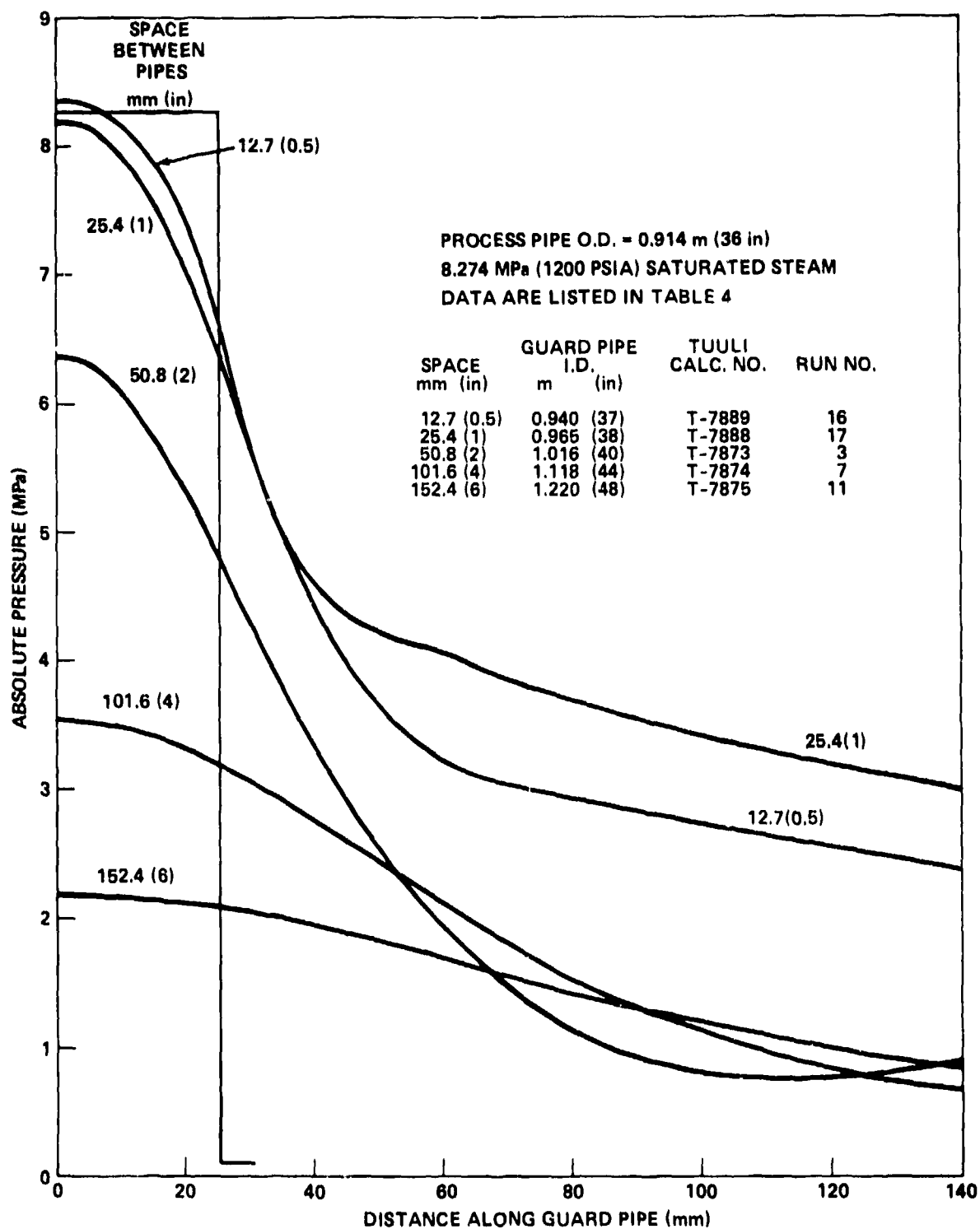
FIGURE 13. STEADY-FLOW PRESSURE ALONG GUARD PIPE FOR 50.8 mm (2 in) LONGITUDINAL BREAK
