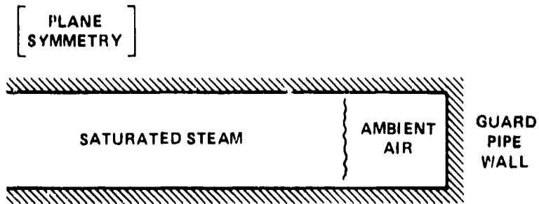
FIGURE 10b. GEOMETRY OF LINEAR SHOCK TUBE PROBLEM
