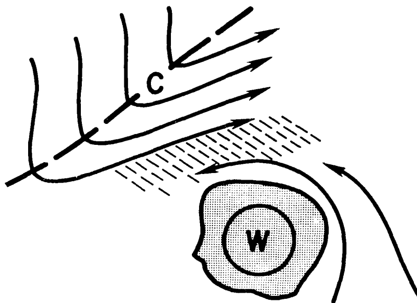
Fig. 57. Schematic representation of how an upper level baroclinic trough to the northwest of a cyclone leads to its weakening. The trough produces an enhanced baroclinic field to the northwest. Simultaneously, a weakening of the storm's cyclonic flow due to momentum mixing in the hashed area would be observed. Such an influence would bring about a thermal wind imbalance such that WS < B . The unbalanced flow mechanism requires that the baroclinicity be reduced and the storm would weaken.
