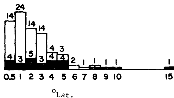
Fig. 80. Distribution of looping diameter in ^{\circ} latitude for the west Pacific (no shading) and for the western Atlantic (shaded).
